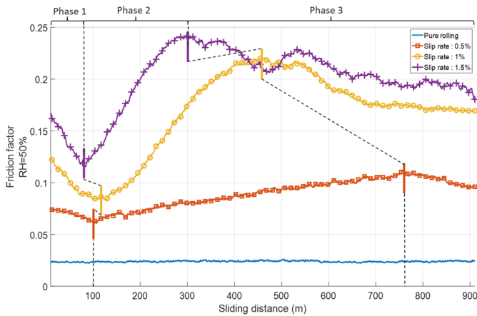
Fig. 12. Friction factor as a function of the sliding distance travelled on Triboring tribometer, plane leaves RH = 50\% . Highlights of the different phases. Phase 1 extends from the beginning of the test to the point where the minimum friction factor is obtained, phase 2 extends to the point where the maximum friction factor is measured, and phase 3 extends to the point where a stabilized friction factor is obtained (corresponding to the end of a test).
