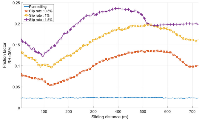
(a) friction factor, RH=35%
