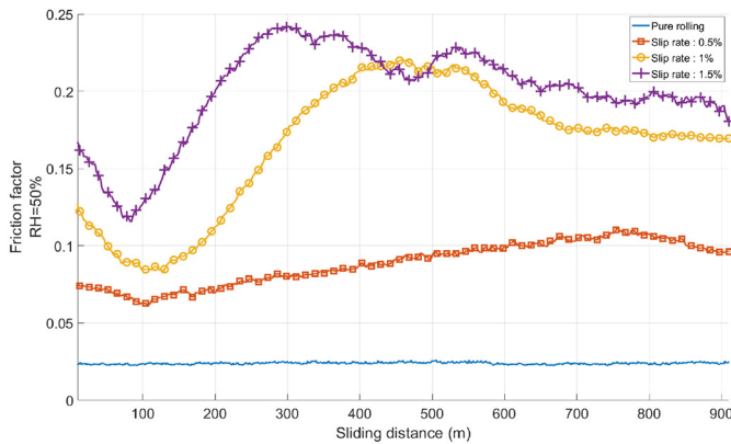
(b) friction factor, RH=50%
