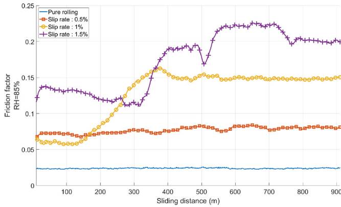
(c) friction factor, RH=85%
