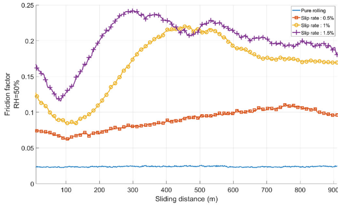
(b) friction factor, RH=50%
