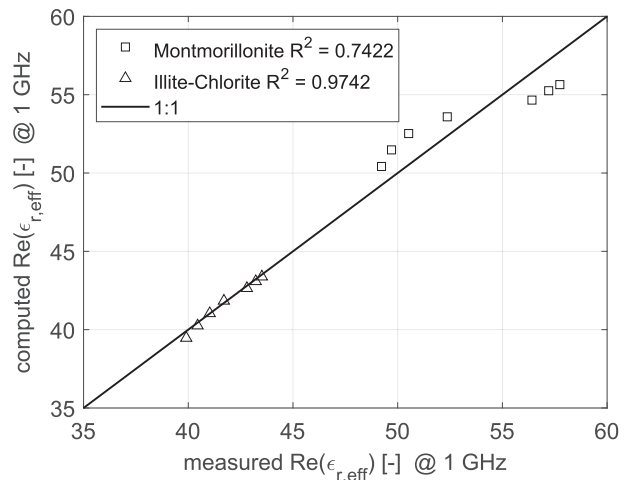
Fig. 9. Computed values versus measured values of Re(\epsilon_{r,eff}) values at f = 10^9 \text{ Hz} for both sample for all measurements.
