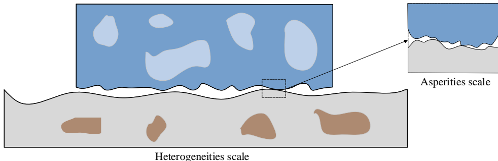
Fig. 1. Double-scale heterogeneities.
