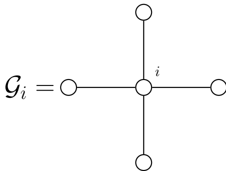
Figure 2. A simply-laced star-shaped graph centred at i (here with 4 peripheral nodes).
