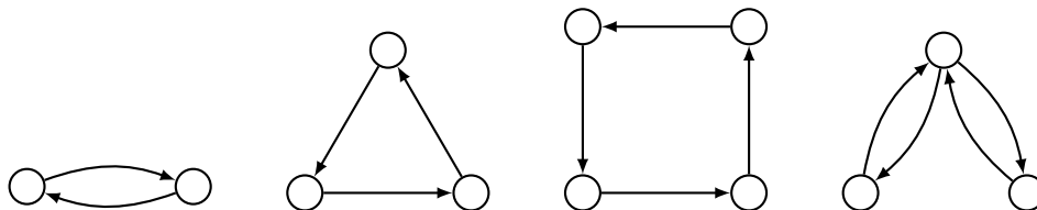
Figure 1. Isomonodromy cycles.
