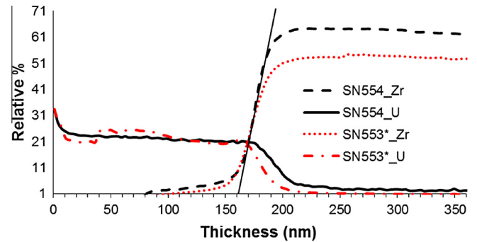
Fig. 11. A plot of the SIMS results for U-Zr pair for samples SN553* (irradiated UO 2 film on YSZ (1 1 0), 5 \times 10^{11} U ions/cm 2 ) and SN554 (unirradiated UO 2 film on YSZ (1 1 0)). U is the film element and Zr is the substrate element.
