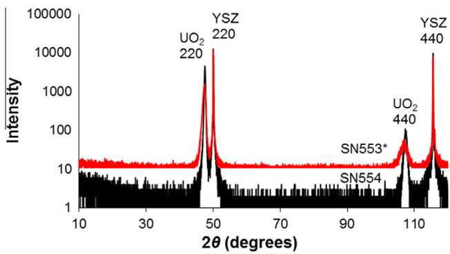
Fig. 6. XRD results for samples SN553* (irradiated \text{UO}_2 film on YSZ (1 1 0), 5 \times 10^{11} ions/cm 2 ) and SN554 (unirradiated \text{UO}_2 film on YSZ (1 1 0)). XRD intensity for irradiated sample SN553* is shifted upwards for clarity.
