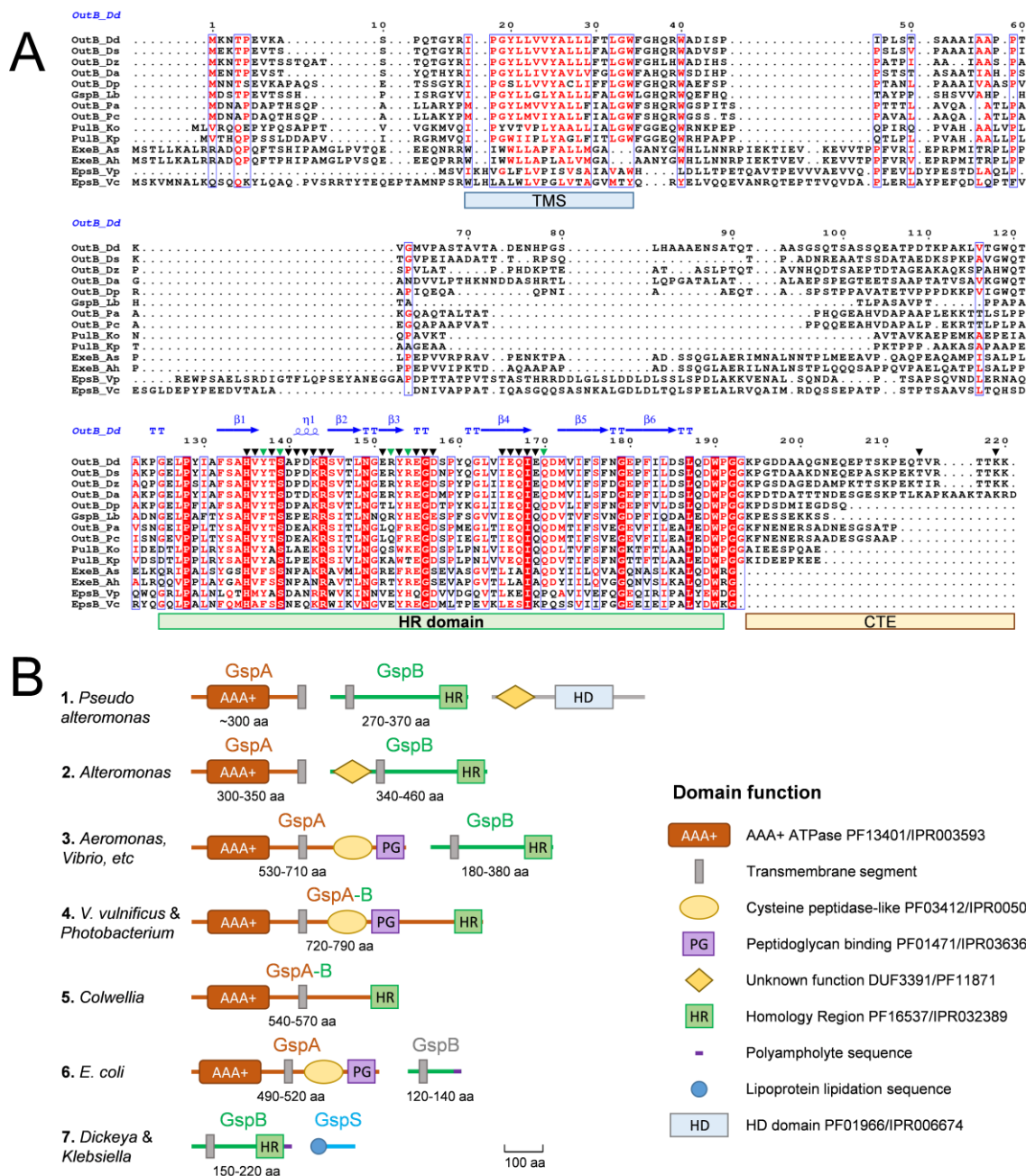
Figure 2. GspB organization. A. Alignment of representative GspB sequences. Multiple sequence alignment was performed with Clustal Omega (ebi.ac.uk) and ESPrpt server (107). The secondary structure elements are shown for the OutB HR domain (PDB entry 4WFW). The residue numbering is this for D. dadantii OutB. The groups of identical and similar residues are highlighted in red or are in red, respectively. The residues substituted with \beta PBA and used in photo-cross-linking are shown with triangles; with green triangles are the residues generating an abundant complex with OutD. Positions of the transmembrane segment (TMS), the homology region (HR) and the C-terminal extension (CTE) are indicated with coloured bars. B. Typical gene and domain organizations of GspB and related GspA and GspS proteins. For each GspB representative shown in Fig. S8A, gene synteny and domain organization were analyzed with NCBI (www.ncbi.nlm.nih.gov), InterPro (www.ebi.ac.uk/interpro) and Pfam (pfam.xfam.org) data bases and summarized into seven archetypes, named according to the most abundant or most studied representative bacterium. The protein size range (in amino acids) is indicated for each group. Of note is that more than 80% of analyzed GspB proteins belong to the archetype #3.
