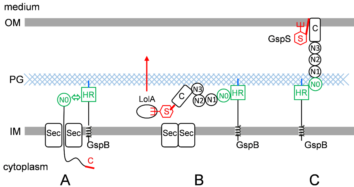
Figure 9. OutB and OutS play complementary functions in targeting, assembly and scaffolding of secretin. A. OutB acts early during OutD export by binding the N0 domain, the first part of the secretin releasing into the periplasm. In this way, OutB could orient the secretin and prevent its mis-insertion into the IM. B. In the later step, pilotin OutS (red hexagon) binds the C-terminal S-domain (red segment) and, with the assistance of the Lol machinery, targets the C-terminal part of the secretin into the OM where several secretin subunits form a channel. C. OutB binds to and stabilizes the N-terminal entry of the secretin channel providing scaffolding with the IM and the PG layer. For simplicity, only one subunit of each protein is shown.
