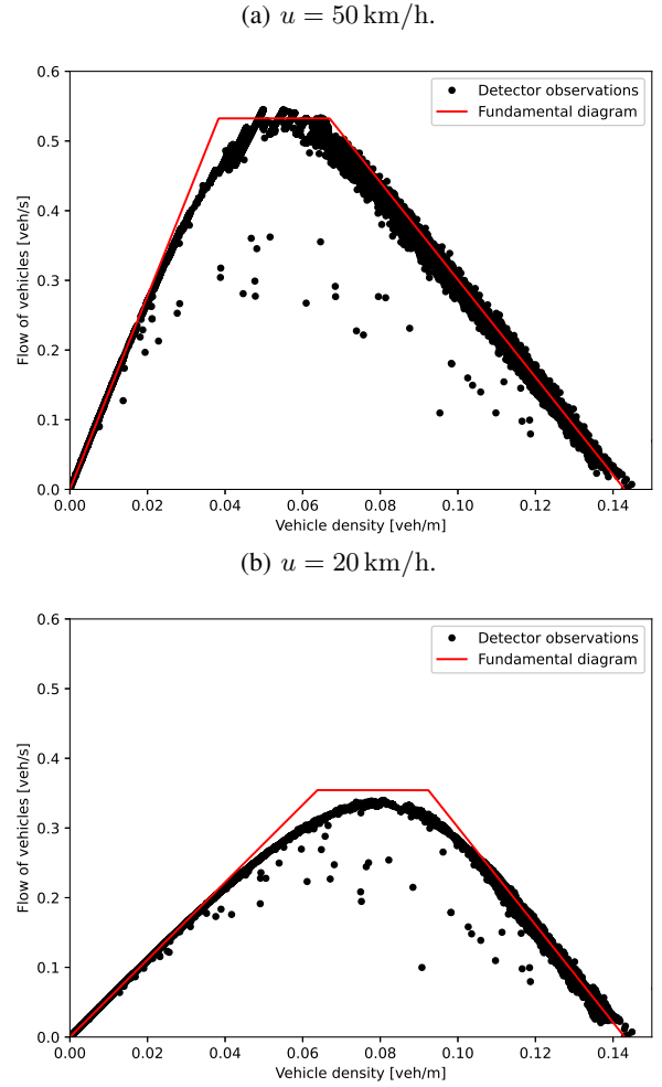
Fig. 2: Fundamental diagrams from ring road simulations, with 50 km/h and 20 km/h speed limits.
