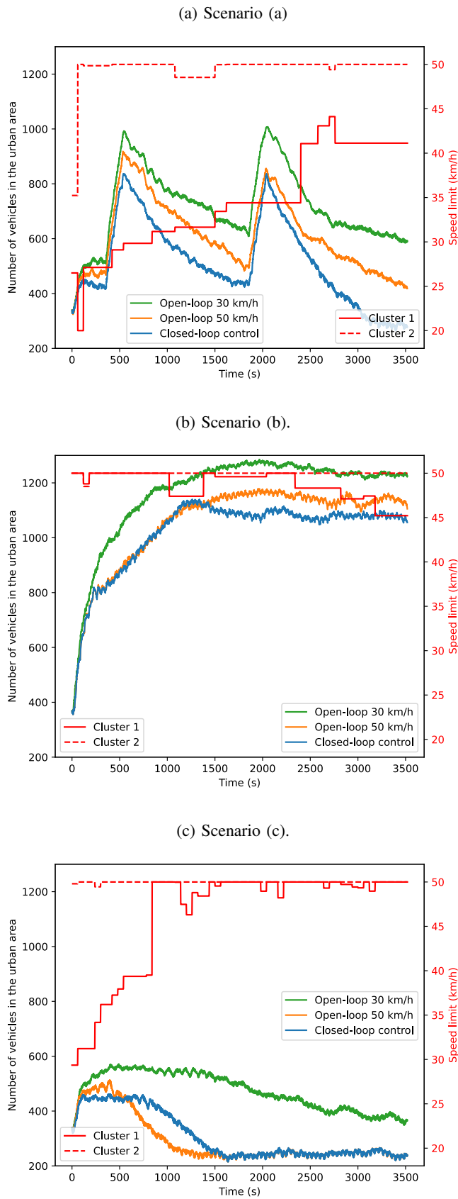
Fig. 9: Evolution of the optimal speed limits in clusters 1 and 2, as well as the number of vehicles in the urban area.
