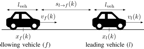
Fig. 1: Representation of the car-following model parameters.
