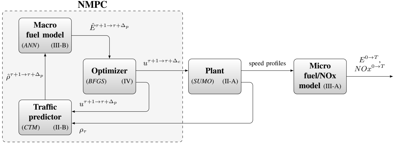
Fig. 5: Block diagram of the global approach for ecological variable speed limits.
