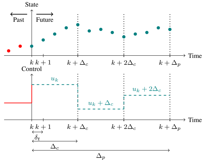
Fig. 6: Representation of the NMPC framework, for \kappa = 3 .
