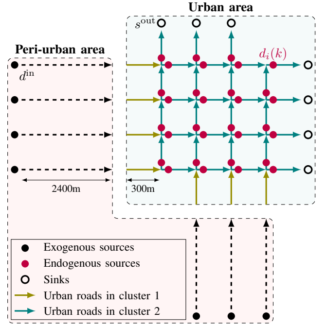
Fig. 7: Road network composed of urban (solid lines) and peri-urban (dashed lines) areas. Urban roads of the same color are in the same cluster and hence have the same speed limit.
