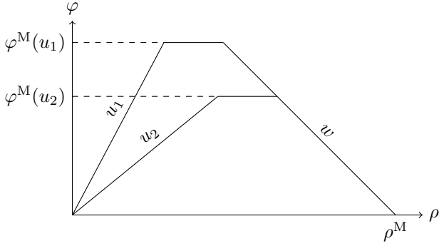
Fig. 3: Fundamental diagrams associated with speed limits u_1 and u_2 , where u_1 > u_2 .
