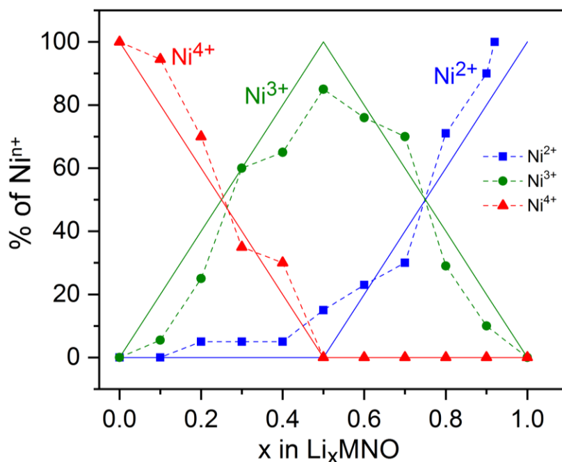
Figure 7. Evolution of the Ni 2+ /Ni 3+ /Ni 4+ ratio during the first discharge of the LiNMO thin film samples. Symbols connected by dashed lines: values obtained from the quantitative analysis of the Raman spectra. Solid lines: expected values derived from the faradaic yield involved during the electrochemical samples preparation.
