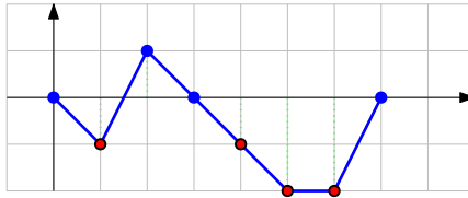
Figure 4. P_c when c = (0, 3, 0, 0, 0, 1, 3) .
