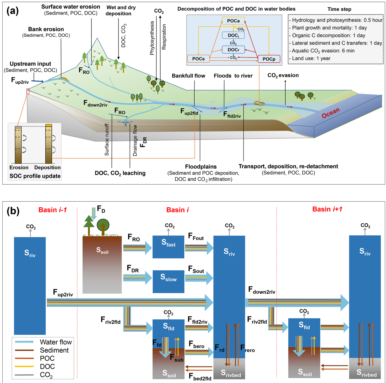
Figure 2. Simulated lateral transfer processes of water, sediment, and carbon (POC, DOC, and CO_2 ) in ORCHIDEE- C_{lateral} (a) and a schematic plot for the reservoirs and flows of water, sediment, and carbon represented in the routing module of ORCHIDEE- C_{lateral} (b). S_{soil} is the soil pool. S_{rivbed} is the sediment (also POC) deposited on the riverbed. S_{fast} , S_{slow} , S_{riv} , and S_{fld} are the “fast”, “slow”, stream, and flooding water reservoir, respectively. F_{RO} and F_{DR} are the surface runoff and belowground drainage, respectively. F_{Fout} and F_{Sout} are the flows from the fast and slow reservoir to the stream reservoir, respectively. F_{up2riv} and F_{down2riv} are the upstream inputs and downstream outputs, respectively. F_{riv2fld} is the output from the river stream to the flooding reservoir. F_{fld2riv} is the return flow from the flooding reservoir to the stream reservoir. F_{bed2fld} is the transformation from deposited sediment in a riverbed to floodplain soil. F_{bero} is bank erosion. F_{rd} and F_{rero} are the deposition and re-detachment of sediment and POC in a river channel, respectively. F_{sub} is the flux of DOC and CO_2 from floodplain soil (originating from the decomposition of submerged litter and soil carbon) to the overlying flooding water. F_{fd} is the deposition of sediment and POC as well as the infiltration of water and DOC. F_D is the wet and dry deposition of DOC from the atmosphere and plant canopy. DOC l and DOC r are the labile and refractory DOC pool, respectively. POC a , POC s , and POC p are the active, slow, and passive POC pool, respectively.
