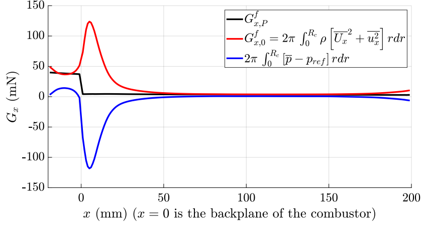
Figure 11: Evolution of G_{x,P}^f and its constituents (Eq. (53)) in the axial direction. The sudden expansion corresponds to x = 0 . The reference pressures are set to p_{ref} = 101\,325.3 Pa in the chamber ( x > 0 ) and p_{ref} = 101\,405 Pa inside the injector ( x < 0 ).
