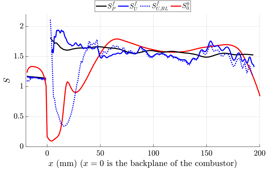
Figure 16: Comparison of 4 formulas for the swirl number.
