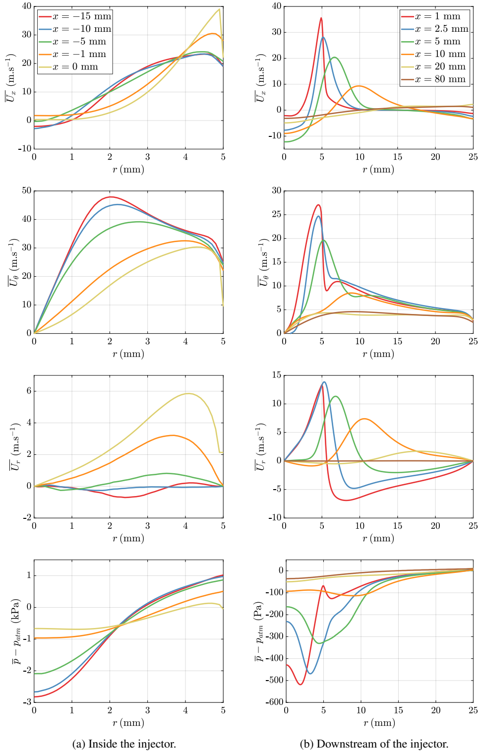
Figure 9: Radial profiles of the mean axial velocity \overline{U}_x , tangential velocity \overline{U}_\theta , radial velocity \overline{U}_r and pressure \overline{p} - p_{atm} . The four plots on the left show these variables for five axial locations inside the injector, the four plots on the right for six axial sections in the chamber.
