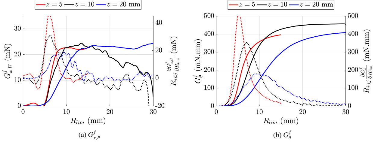
Figure 20: Effect of integration limit on the estimated flow rates G_{x,U}^f (left, plain line) and G_\theta^f (right, plain line) at z = 5, 10 and 20 mm. The integral terms are computed by stopping the integration at various distances R_{lim} . As recommended in appendix B, the derivative with regards to R_{lim} of the momentum flowrates are shown as dotted lines. They are multiplied by the radius of the injector R_{inj} for scaling.
