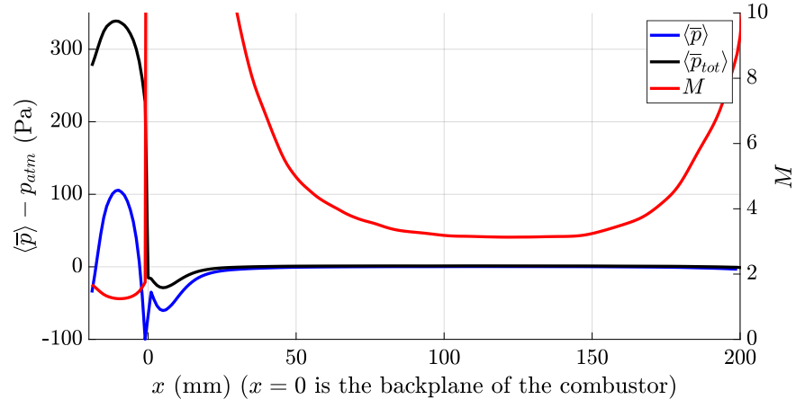
Figure 23: Axial evolution of the section averaged static (blue) and total (black) pressure \langle \bar{p}_{tot} \rangle = \langle \bar{p} + 1/2 \rho (\overline{U^2} + \overline{u^2}) \rangle in the system (left axis). The atmospheric pressure p_{atm} = 101\,325 Pa is removed. Values of the Boussinesq momentum coefficient M (red) are given in the right axis.
