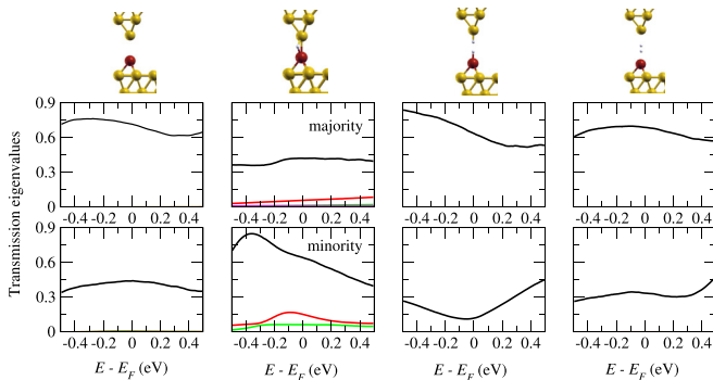
FIG. 13. Transmission eigenchannels for Fe, FeH 1 , FeH 2 perp I, and FeH 2 perp II close to contact. Colors indicate different transport channels. Only FeH 1 shows multichannel transport behavior.
