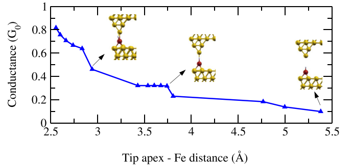
FIG. 11. Conductance variation during the approach process for \text{FeH}_1 contacts. A clear conductance plateau is observed.
