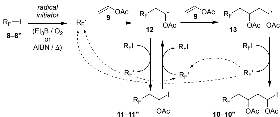
Scheme 7. Mechanism of formation of mono- and bis -adducts 11–11'' and 10–10'' from R_F-I and vinylacetate through (iodine) atom-transfer radical chain reaction.
