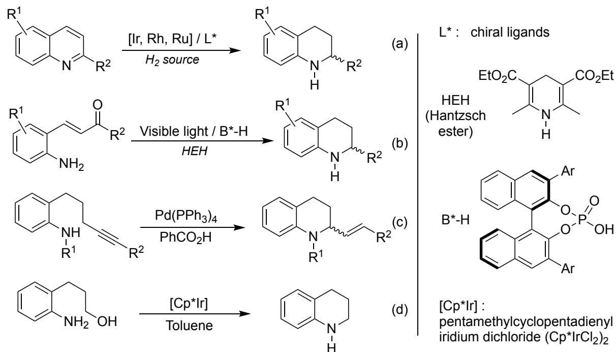
Scheme 3. Examples of catalytic syntheses of 1,2,3,4-THQ. 17–21
