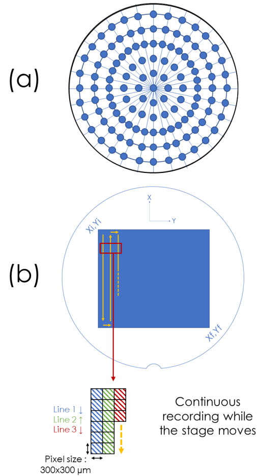
Fig. 4 – (a) Typical mapping used for point-to-point basic measurements and (b) Raster scanning scenario of the wafer, local dense pixelization with the 300x300 μm spot and full dense scan of a large area with 300x300 μm recorded “pixels”.
