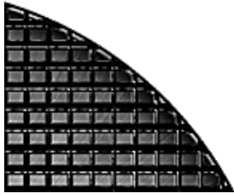
Fig. 12 – Reflectometry image exhibiting the striations signature
