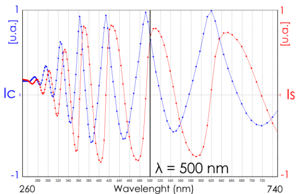
Fig.8 – I_c and I_s spectroscopic scan on the blanket wafer for the wavelength selection protocol
