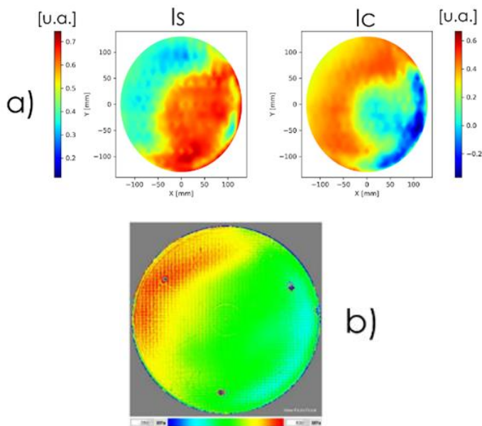
Fig.11 – a) Model-less ellipsometry images at 338nm (6000 points) and b) Interferometry stress cartography of nitride layer deposited on patterned wafer.
