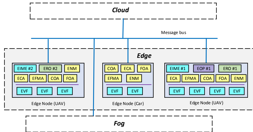
Figure 6. VMCS architecture.
