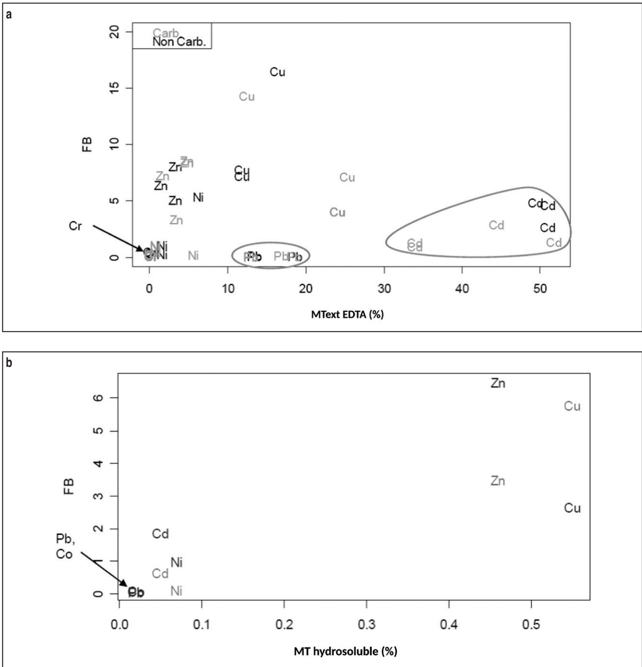
Figure 5: Relationship between the bioaccumulation factor (BF) of springtails and the percentage of TM associated with (a) the EDTA-extractable fraction in the soil surface horizon for carbonate (in gray) and non-carbonate (in black) soils for the different TMs (n = 42); (b) the water-soluble fraction of soils extracted according to Leleyter and Probst (1999) for samples from the Auradé watershed (AUR7 and AUR8). The values of profile 7 (AUR7, under wheat) are indicated in gray and those of profile 8 (AUR8, under forest) are indicated in black (n = 10).
