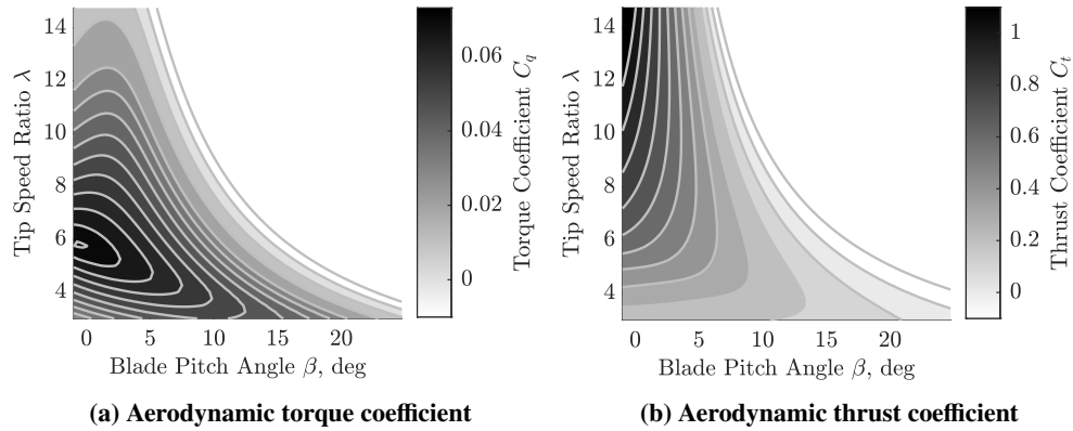
Fig. 2 Thrust and torque coefficients as a function of the pitch angle and the tip-speed ratio.
