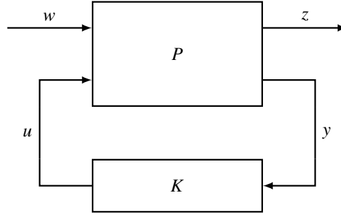
Fig. 4 Closed loop system configuration for the structured H_\infty problem formulation.
