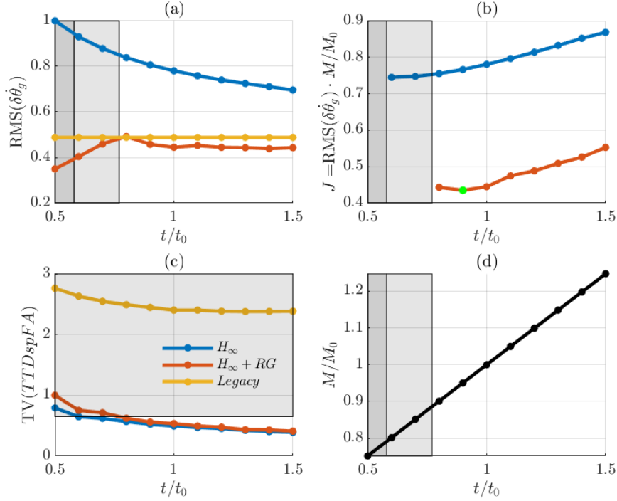
Fig. 7 Control co-design optimization problem. (a) RMS of delta generator speed. (b) Cost function. (c) TV of tower top deflection. (d) Wind turbine mass to reference mass ratio.
