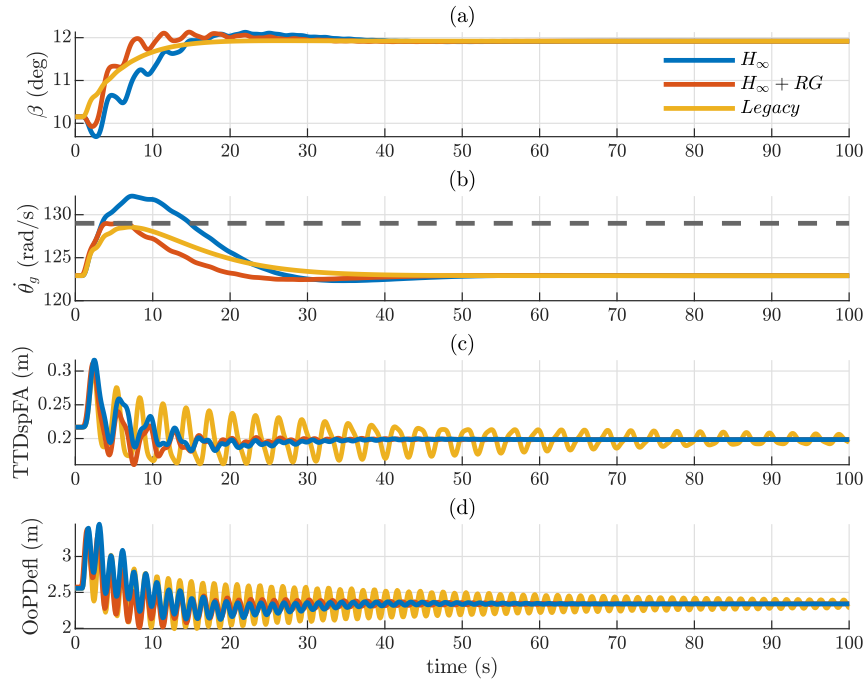
Fig. 6 Time response to a 1-m/s step input in wind speed for a land-based wind turbine. (a) Blade-pitch angle. (b) Generator speed. (c) Tower top fore-after deflection. (d) Blade tip out-of-plane deflection.
