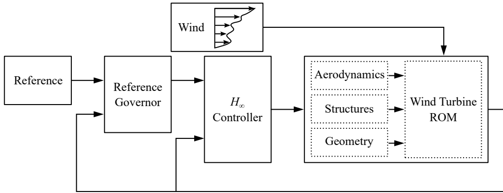
Fig. 5 Reference governor applied to closed loop system.
