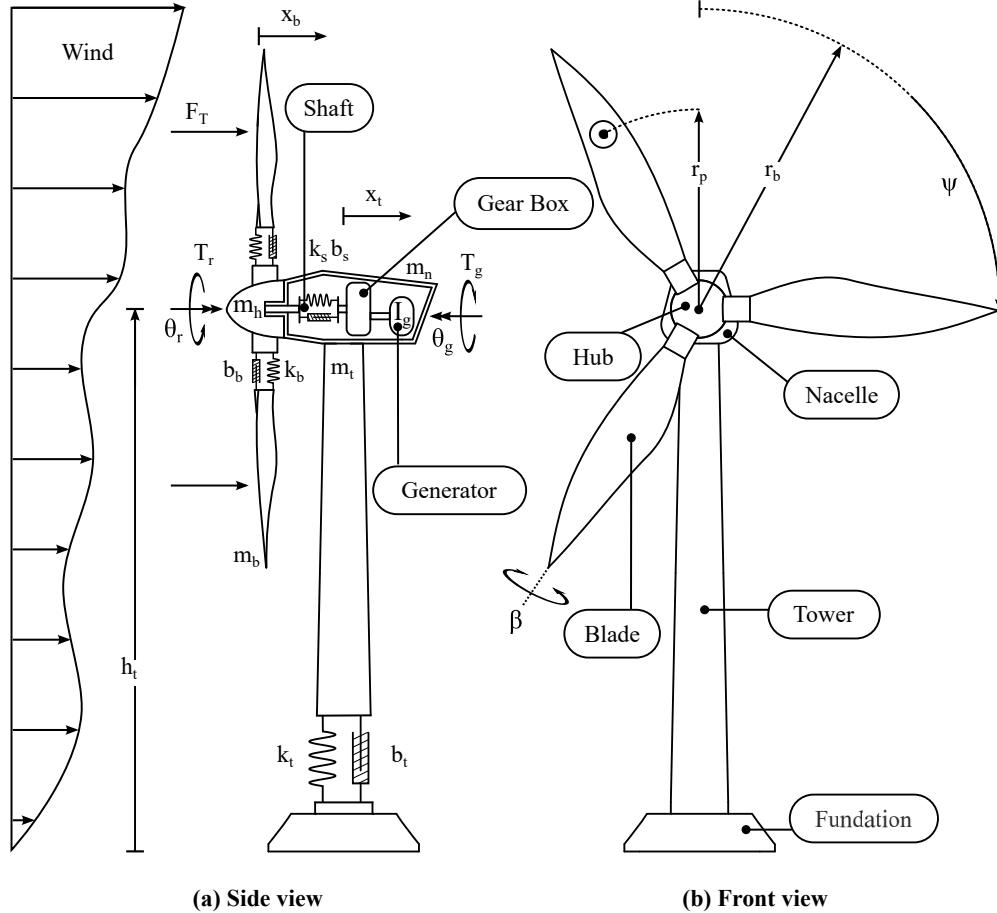
Fig. 1 Assumed model of the wind turbine including the rotor, the drive-train, the generator, and the tower.
