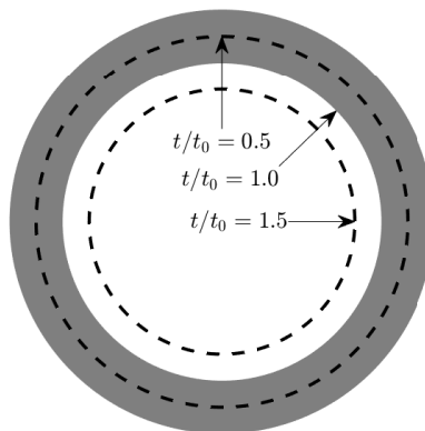
Fig. 3 Hollow cylindrical cross-section of the wind turbine tower.
