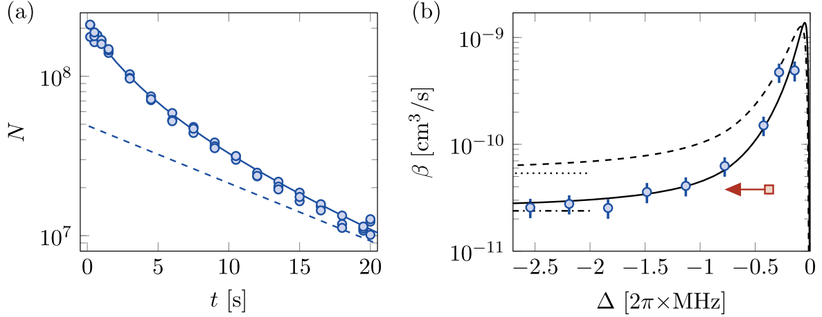
Figure 6. (a) Decay of the atom number with time for a laser detuning \Delta = -2\pi \times 2.54 MHz, a saturation parameter s = 0.65 and a gradient G = 1.71 G cm -1 . The data is fitted with a solution of the decay model (10) (solid line), leading to a two-body loss coefficient \beta = 2.3(5) \times 10^{-11} cm 3 s -1 . The dashed line corresponds to the exponential asymptote associated with one-body atom losses ( 1/e time constant \tau_1 = 12 s). (b) Variation of the loss coefficient \beta with the detuning \Delta , compared with the predictions of the molecular dynamics model. The dashed line corresponds to molecular parameters \lambda = \bar{\lambda} and \mu = \bar{\mu} , while the solid line is a fit with \lambda and \mu being free parameters. The dotted and dashed-dotted lines stand for the corresponding asymptotic expression (12). The red square corresponds to the decay coefficient measured in [15], with the arrow indicating the required detuning renormalization (see text).
