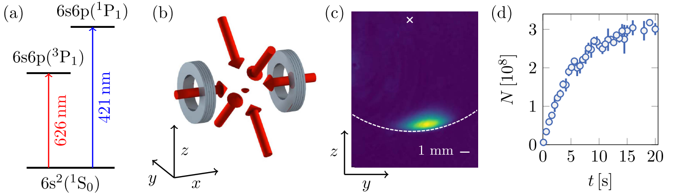
Figure 1. (a) Scheme of the optical transitions involved in our laser cooling setup, coupling the electronic ground state 4f^{10}(^5I_8)6s^2(^1S_0) ( J=8 ) to the excited states 4f^{10}(^5I_8)6s6p(^1P_1)(8,1)_9 ( J'=9 ) and 4f^{10}(^5I_8)6s6p(^3P_1)(8,1)_9 ( J'=9 ). (b) Scheme of the magneto-optical trap arrangement, with the six MOT beams (red arrows) and the pair of coils in anti-Helmholtz configuration. Gravity is oriented along -z . (c) Typical in situ absorption image of an atomic sample held in the ‘compressed’ magneto-optical trap. The cross indicates the location of the quadrupole center. The cloud is shifted by \sim 1 cm below the zero due to gravity. We attribute the cloud asymmetry with respect to the z axis to the effect of an ambient magnetic field gradient. (d) Atom number N captured in the magneto-optical trap as a function of the loading time t (see text for the MOT parameters).
