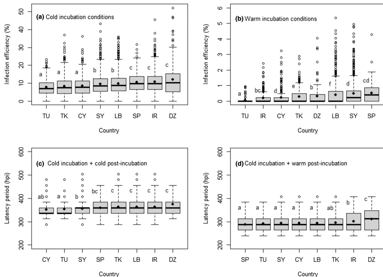
FIGURE 3 Infection efficiency (%) of 26 Puccinia striiformis f. sp. tritici isolates classified by country of origin for cold incubation (5°C) and for warm incubation (20°C) temperature (a, b), and latency period (hours postinoculation, hpi) for cold incubation temperature (5°C) and cold postincubation (10°C/15°C) versus warm postincubation (16°C/25°C) temperature regime (c, d). CY: Cyprus, DZ: Algeria, IR: Iran, LB: Lebanon, SP: Spain, SY: Syria, TK: Turkey, TU: Tunisia.
