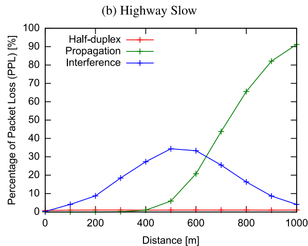
FIGURE 7. Percentage of Packet Loss (PPL) as a function of transmitter-receiver distance.
