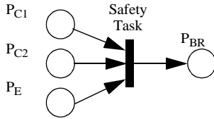
Fig. 6. Petri net model of the safety function
