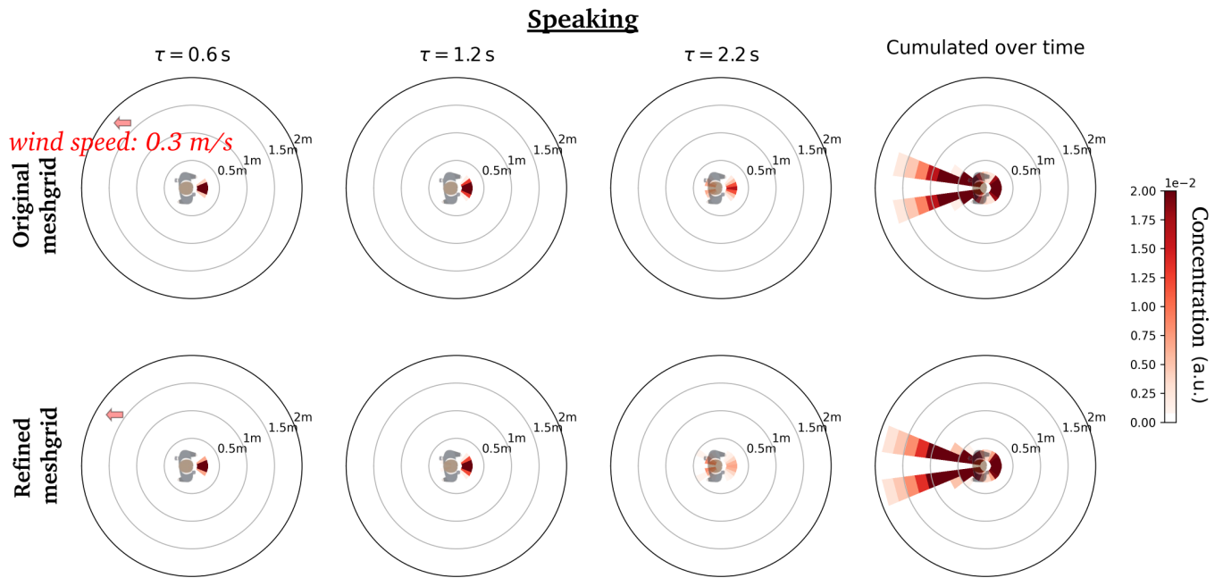
FIG. S2. Comparison of the dynamic concentration maps generated at distinct time delays \tau for a static pedestrian in a head wind blowing at 0.3\text{ m}\cdot\text{s}^{-1} , by coarse-graining CFD simulations performed with ( top row ) the original meshgrid, ( bottom row ) a refined meshgrid.
