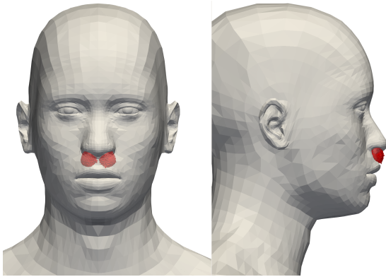
FIG. S6. Region of the simulation domain where the vertical air flow during inhalation reaches a speed of at least 0.3 \text{ m} \cdot \text{s}^{-1} , as required to compensate the downward sedimentation of droplets of diameter about 100 \mu\text{m} . The inhaling flow rate is 0.55 \text{ L s}^{-1} .
