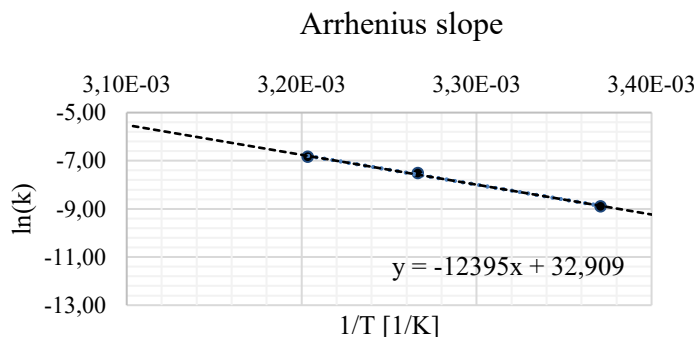
Figure 4: Arrhenius slope
