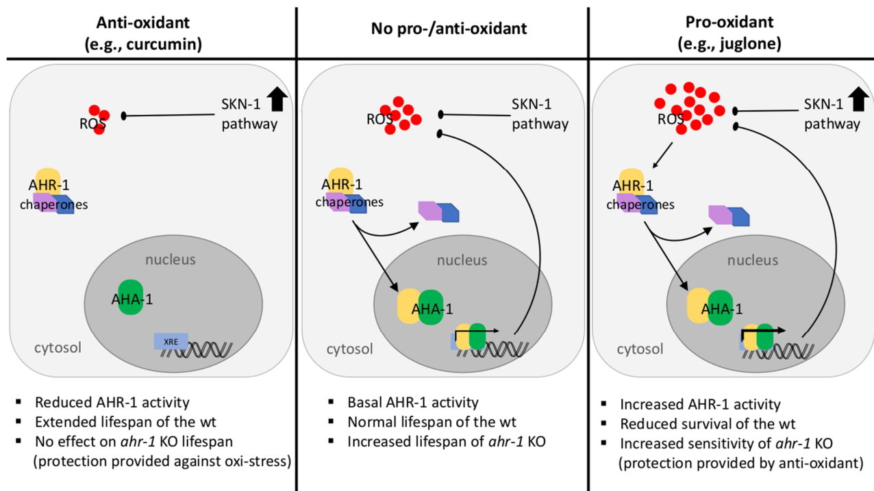
Figure 7. Proposed model of the AHR-1 signaling pathway in C. elegans response to pro- and antioxidants. In “normal” conditions (middle panel), AHR-1 is activated by intra-cellular ROS. This leads to the shedding of the chaperones from cytosolic AHR-1 and the subsequent nuclear translocation of AHR-1. In the nucleus, AHR-1 forms a heterodimer with the AHR nuclear translocator (AHA-1) and bind to XREs of target genes, which in turn leads to the reduction in intracellular ROS levels. In these conditions, loss of ahr-1 function leads to an increased lifespan. In the presence of antioxidants (left panel) the intra-cellular ROS concentrations are low leading to AHR-1 residing in the cytoplasm, bound by its cofactors. The inhibition of the basal AHR-1 activity leads to an increased lifespan. In the presence of pro-oxidants (right panel) AHR-1 is activated by excessive ROS, which results its nuclear translocation, the AHR-1–AHA-1 heterodimer formation and the initiation of target gene transcription. In the ahr-1 KO, the decreased detoxification of ROS through AHR-1-induced target genes leads to an accumulation of ROS and renders the ahr-1 KO susceptible.
