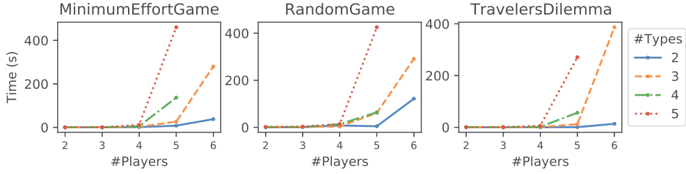
Fig. 3. Avg. execution time (s), MILP-PNE, for the games that admit a PNE, |A_i| = 2 , n \in [2, 6] , |\Theta_i| \in [2, 5] . Missing configurations (e.g. 6 players/5 types for the three categories of games) are configurations where no game with a PNE was found.
