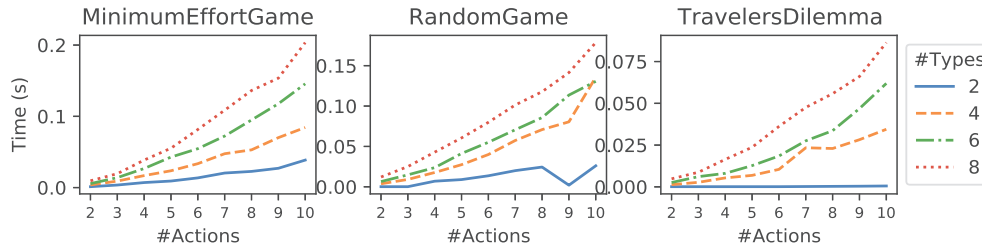
Fig. 6. Avg. execution time (s) to find a \Pi -MNE, n = 2 , |A_i| \in [2, 10] , |\Theta_i| \in [2, 8] .
