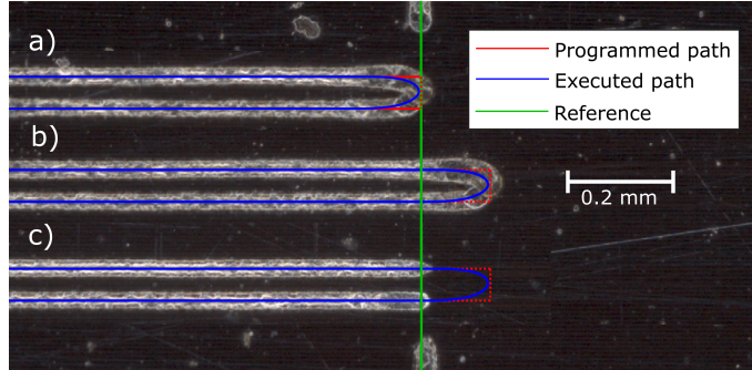
Figure 6: Melt tracks on the substrate, a) without compensation vectors, b) with compensation vectors ( 130 \mu\text{m} ) but wrong laser parameters, c) with compensation vectors ( 130 \mu\text{m} ) and correct laser parameters
