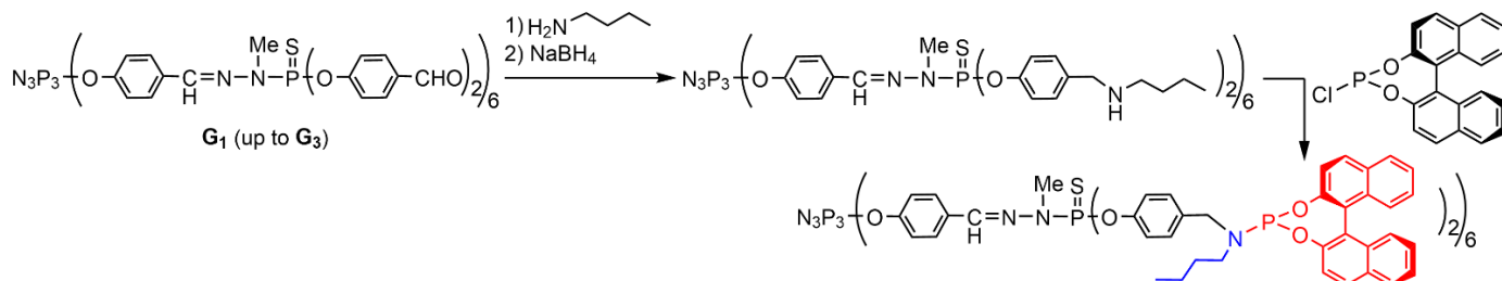
Scheme 12. Grafting of an aminophosphoramidite ligand on the surface of PPH dendrimers. The Rh complexes efficiently catalyzed [2+2+2] cycloadditions.
