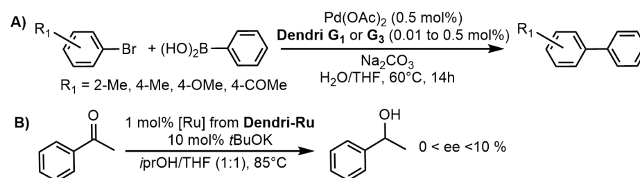
Figure 4. (A) Suzuki coupling catalyzed by Pd complexes of the dendrimers shown in Scheme 4A. (B) Transfer hydrogenation catalyzed by Ru complexes of the dendrimers shown in Scheme 4B.
