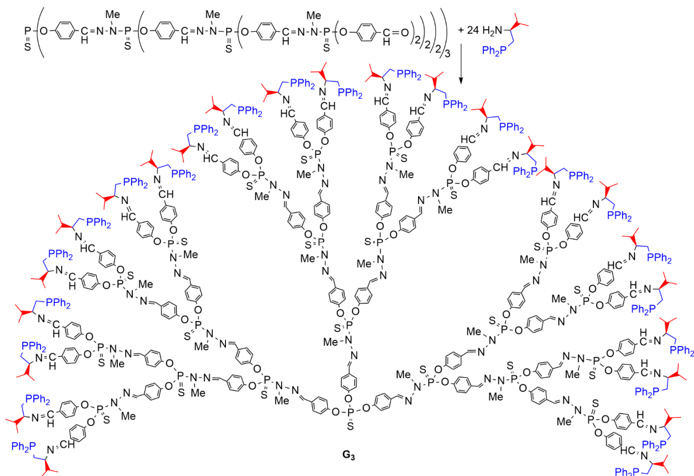
Scheme 3. Synthesis of the 3rd generation of a PPH dendrimer decorated with chiral iminophosphine end groups. The Pd complex was used as catalysts in asymmetric allylic alkylation.
