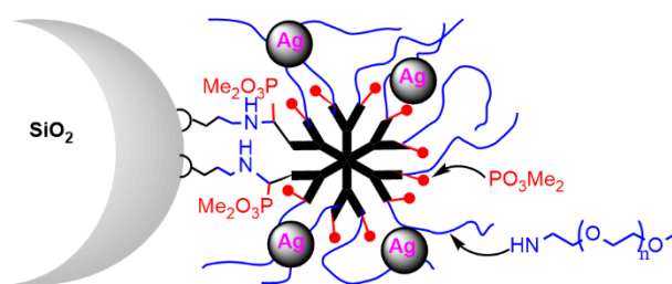
Figure 8. Dendrimers linked to SiO 2 NPs and hosting Ag/Ag 2 O NPs exhibiting antibacterial activity.
