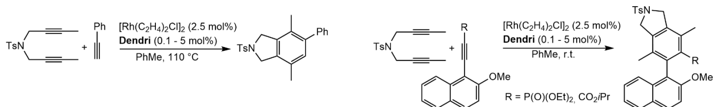
Figure 7. [2+2+2] cycloaddition reactions catalyzed by the Rh complex of the dendrimers shown in Scheme 12.
