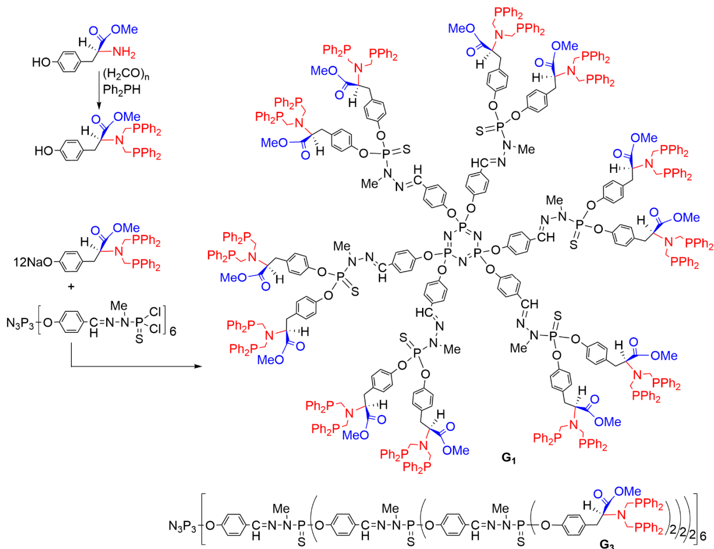
Scheme 5. Synthesis of the 1st generation of PPH dendrimer bearing diphosphine derivatives of L-tyrosine methyl ester as terminal functions, and linear representation of the corresponding third generation. The palladium complexes were used as catalysts in C-C cross-coupling reactions.
