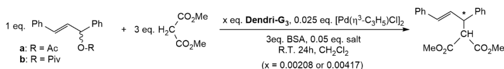
Figure 3. Allylic alkylation catalyzed by the Pd complex of the G 3 dendrimer shown in Scheme 3.
