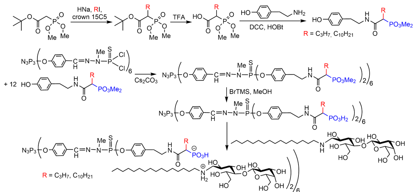
Scheme 8. Synthesis of phosphonate dendrimers bearing a pendant alkyl chain and a phosphonic acid, and their association with a derivative of galactosylceramide, having anti-HIV properties.
