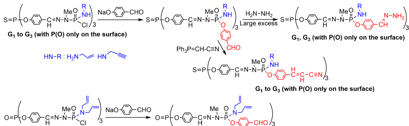
Scheme 19. Sequential addition of an amine and of 4-hydroxybenzaldehyde on the surface of PPH dendrimers.
