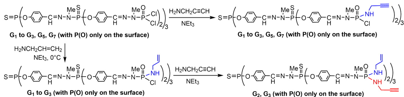
Scheme 17. Sequential addition of two different amines on the surface of polyphosphorhydrazone dendrimers having P(O)Cl 2 terminal functions.
