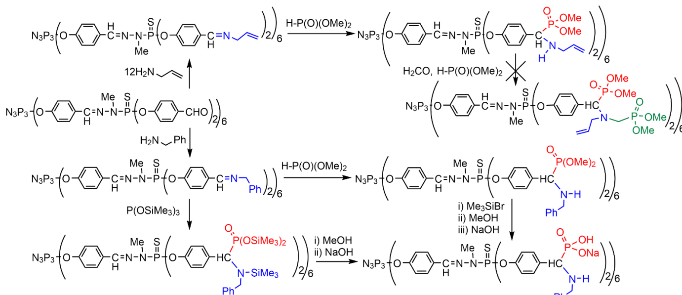
Scheme 13. Two-step processes from aldehydes, affording phosphonate and secondary amines as terminal functions of PPH dendrimers. They display poor anti-inflammatory properties.
