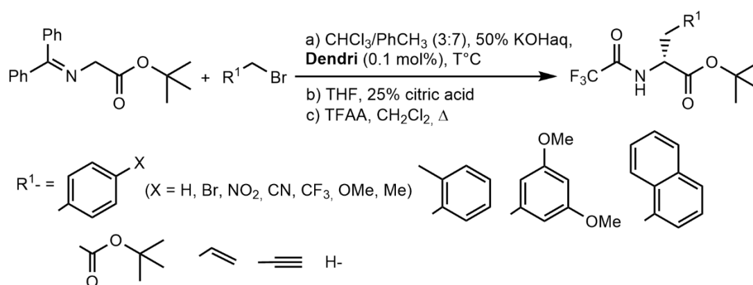
Figure 6. Asymmetric alkylation of a glycinate Schiff base with different types of bromides, in particular benzylbromide derivatives, organocatalyzed with the dendrimer functionalized with (+)-cinchonine, as shown in Scheme 6.
