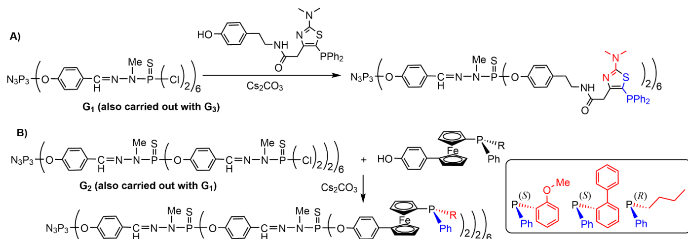
Scheme 4. Synthesis of dendrimers functionalized with thiazolyldiphenylphosphine for which the Pd complex was used in Suzuki couplings (A) and chiral ferrocenylphosphines for which the Ru complexes were used in switchable transfer hydrogenations (B).
