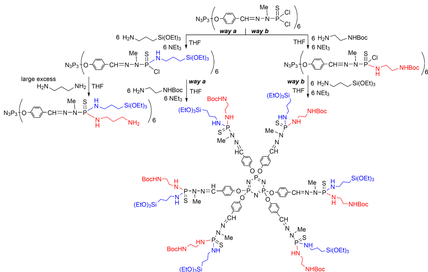
Scheme 18. Other examples of sequential addition of two different amines on PPH dendrimers, to be grafted to silica, and used for trapping CO 2 .
