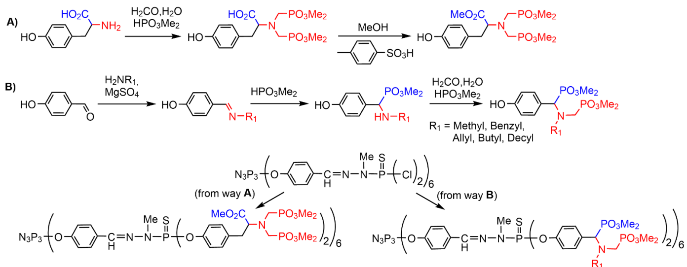
Scheme 9. Synthesis of bifunctional phenols from tyrosine (way A) and from 4-hydroxybenzaldehyde (way B), and structure of 1st generation of PPH dendrimers modified with them. The anti-inflammatory properties of these dendrimers were then tested.
