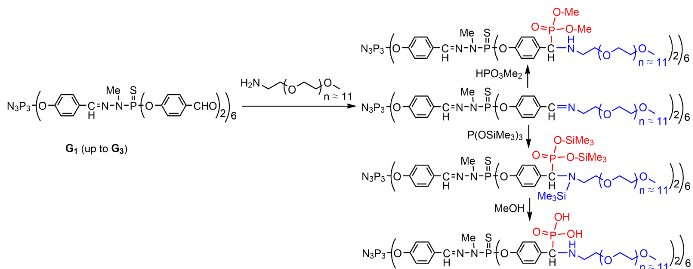
Scheme 14. Two different routes for the synthesis of a series of \alpha -amino-PEG-phosphonate-terminated PPH dendrimers, having very low cytotoxicity.
