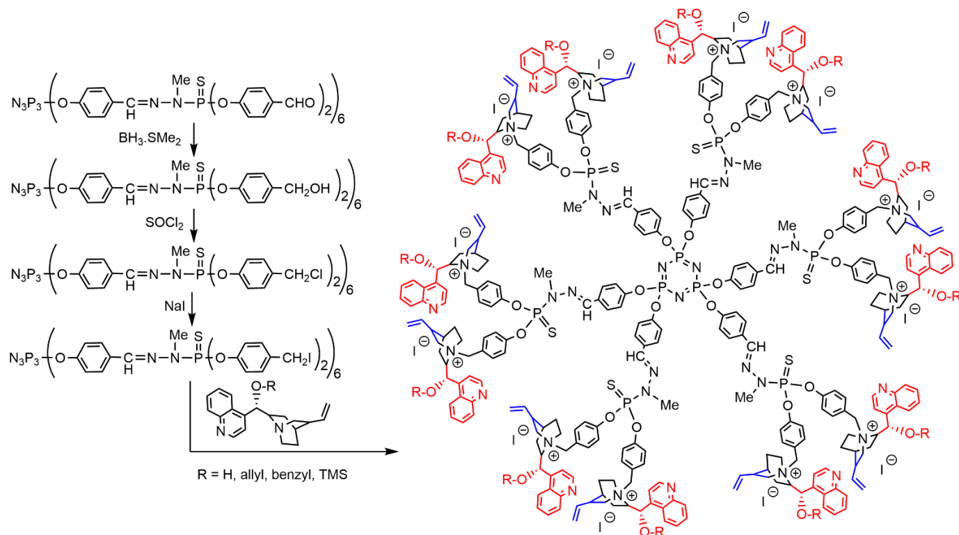
Scheme 6. Modification of the surface of a first generation PPH dendrimer for enabling the alkylation of the quinuclidinic N atom of several types of (+)-cinchonine, used as organocatalysts.
