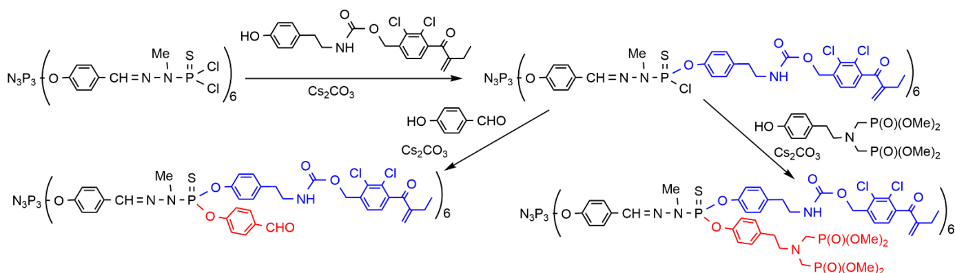
Scheme 21. Grafting of a phenol derivative of ethacrynic acid and other phenols on the surface of PPH dendrimers having anticancer properties.
