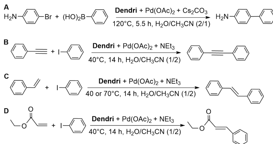
Figure 5. Catalytic reactions carried out with Pd complexes of the dendrimers shown in Scheme 5. (A) Suzuki coupling; (B) Sonogashira coupling; (C,D) Heck couplings.
