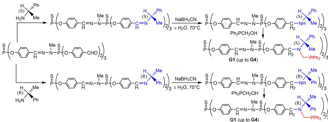
Scheme 11. Two-step method for the grafting of two terminal groups from aldehydes.
