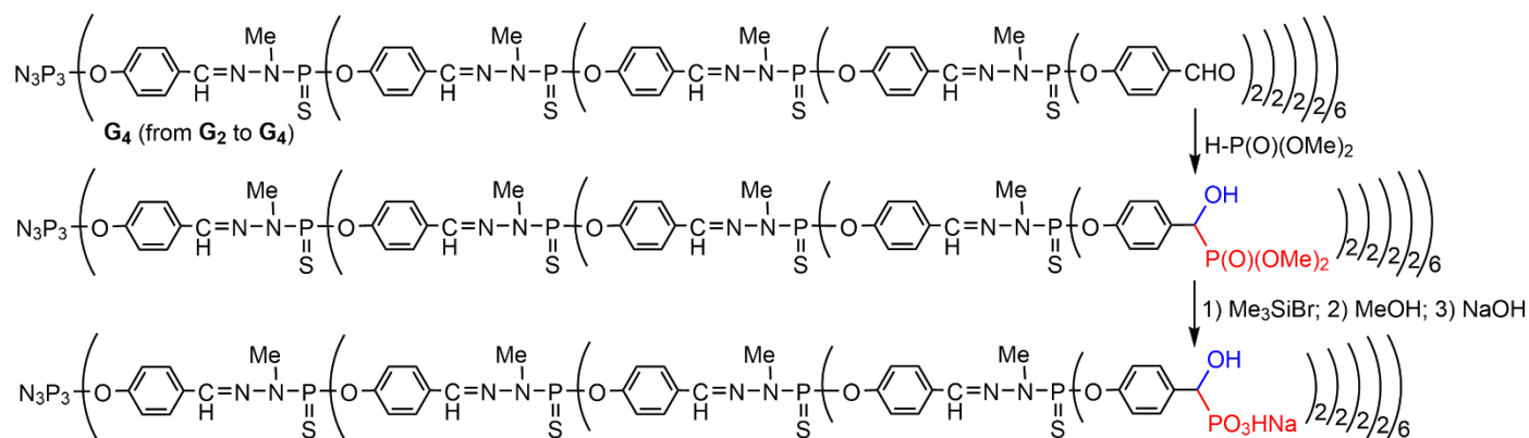
Scheme 15. Direct addition of H-P(O)(OMe) 2 on aldehyde terminal functions. These dendrimers efficiently controlled the mineralization of Ti(OiPr) 4 .
