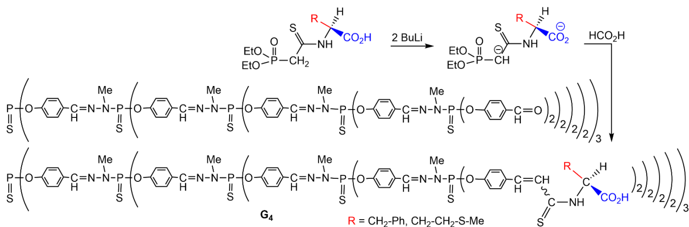
Scheme 2. Generation 4 PPH dendrimer functionalized with amino acid terminal functions, obtained by Horner-Wadsworth-Emmons reactions on aldehyde terminal groups.
