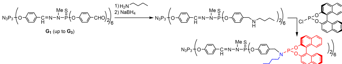
Scheme 12. Grafting of an aminophosphoramidite ligand on the surface of PPH dendrimers. The Rh complexes efficiently catalyzed [2+2+2] cycloadditions.
