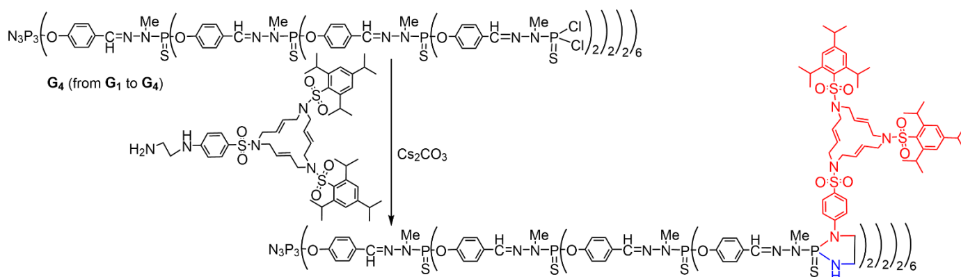
Scheme 7. Grafting of 15-membered macrocycles, suitable for creating branched supramolecular assemblies of Pt nanoparticles.
