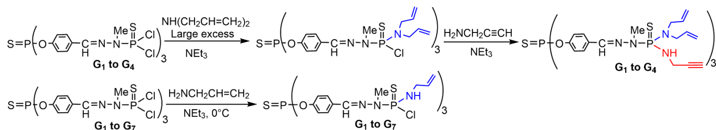
Scheme 16. Sequential addition of two different amines on the surface of PPH dendrimers.
