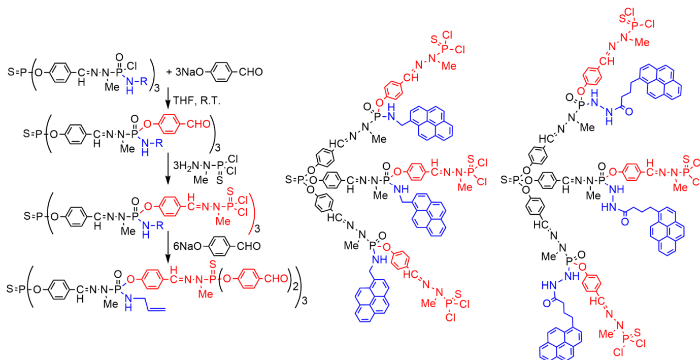
Scheme 20. Amino derivatives of allyl or pyrene as pendant functions inside polyphosphorhydrazone dendrimers.
