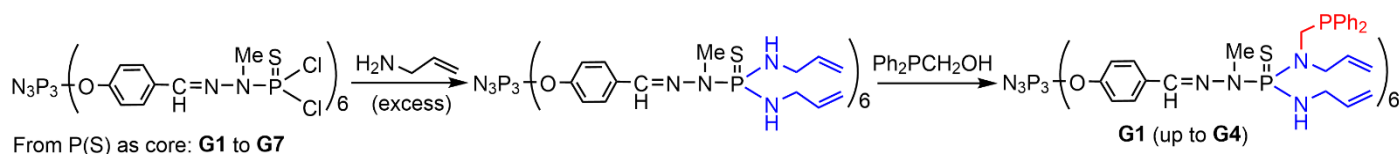
Scheme 10. Grafting of diphenylphosphine as the second functional group to PPH dendrimers.
