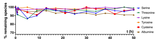
Figure 4. Stability of carbamoyl fluoride 1a in presence of various nucleophilic amino-acids and serum albumin (T = 28°C).
