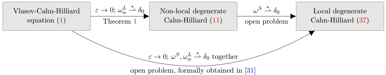
Figure 1: Relation between three types of the degenerate Cahn-Hilliard equations.
