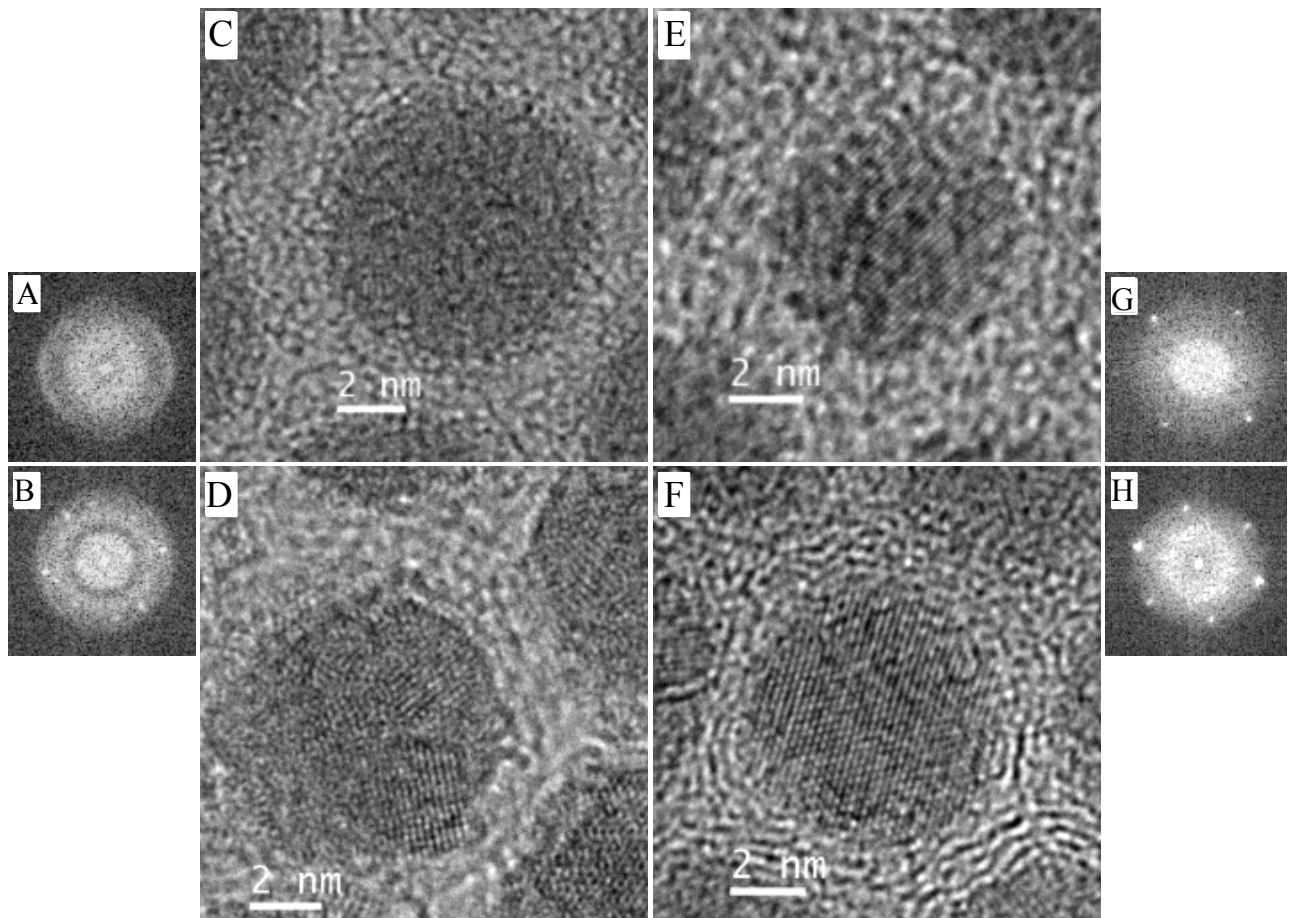
Figure 3. Power spectra and HRTEM images of a Co polycrystal: after 0 min (A and C) and 16 min of irradiation (B and D) and an hcp-Co single-crystal: after 0 min (E and G) and 16 min of irradiation (F and H). NCs are selected from the Figure 2.
