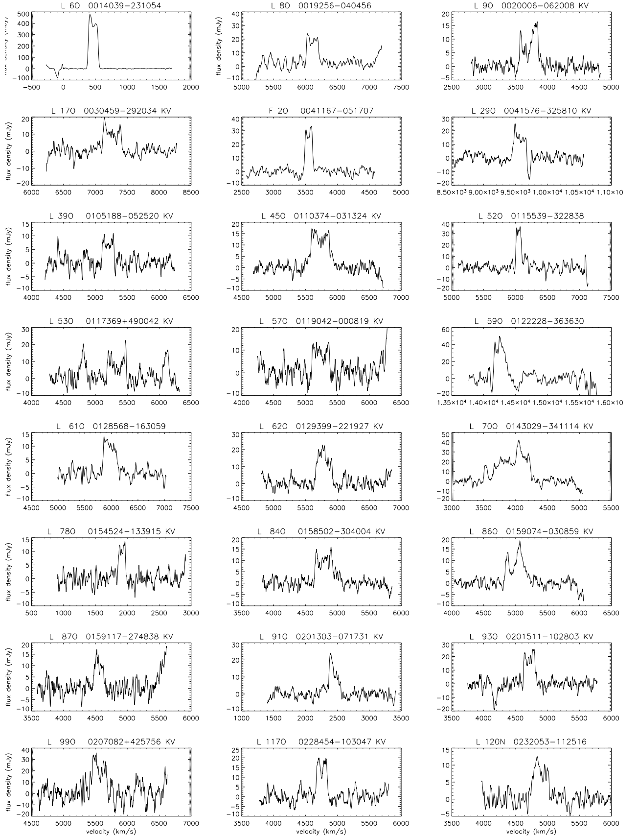
Fig. 1. a) Nançay 21-cm HI line spectra of detected objects (see Table 3). Velocity resolution is 15.8 \text{ km s}^{-1} (velocity search mode) and 17.1 \text{ km s}^{-1} (known velocity mode), radial heliocentric velocities are according to the optical convention. Galaxies detected in the “known velocity” mode are indicated by the designation “KV” following their coordinates in the header of their spectrum.
