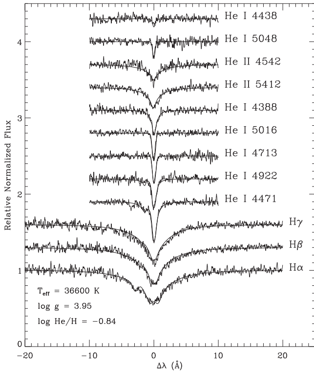
Figure 4. Best-fitting model plotted over the Balmer, He I, and He II lines observed in the Keck HIRES spectrum of \nu Z 1128. The faint absorption feature in the blue wing of H\alpha is the He II \lambda 6560 line. The He I \lambda 5875 line is not detected in the HIRES spectrum, because the line is located in a gap between two spectral orders. The He II \lambda 4686 line is not shown, because the line is corrupted by an artefact and is not usable by the fitting procedure.
