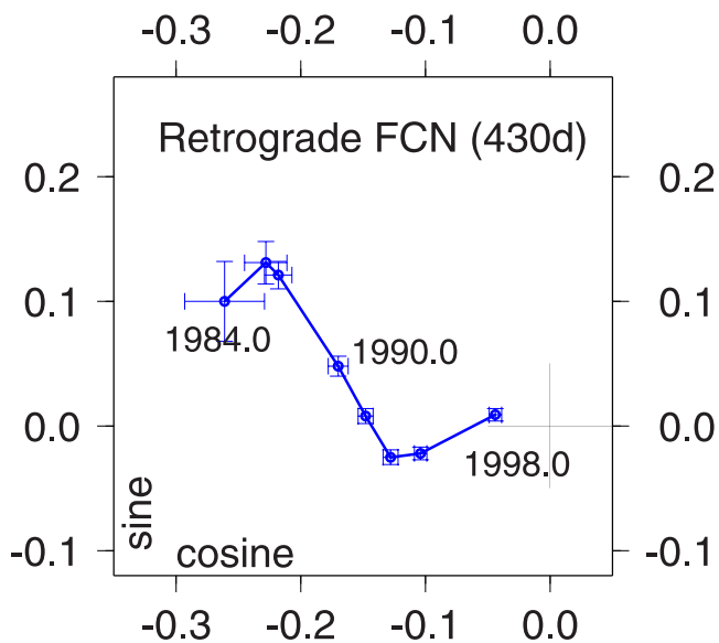
Figure 3. VLBI-derived retrograde component at the FCN frequency (430 days). The origin of phases is J2000.0. Unit is mas.
