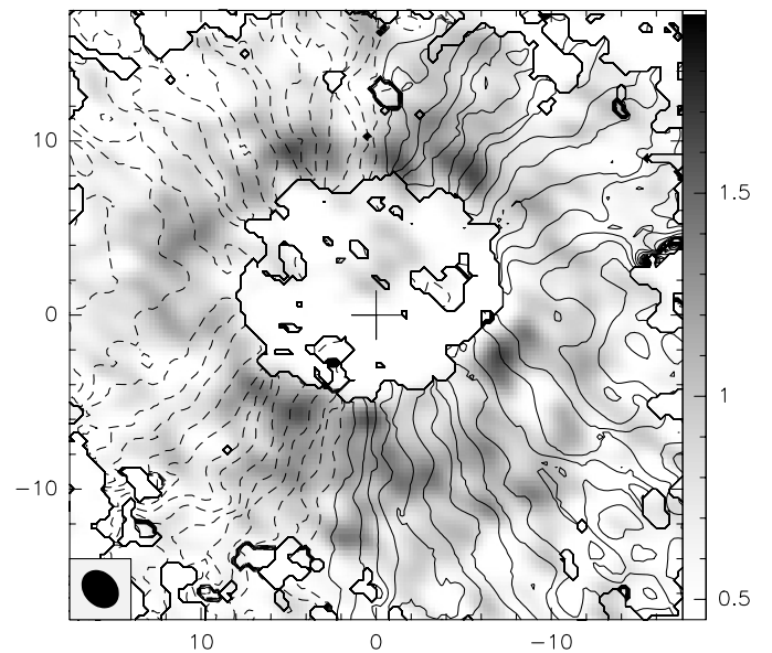
Fig. 6. Overlay of the integrated intensity map of CO(1–0) (in gray scale) with the CO mean-velocity field, in contours spanning the range -150 \text{ km s}^{-1} to 150 \text{ km s}^{-1} in steps of 10 \text{ km s}^{-1} . Velocities are referred to V_{\text{hel}} = 952 \text{ km s}^{-1} . Solid (dashed) lines are used for positive (negative) velocities. The first solid contour represents systemic velocity.
