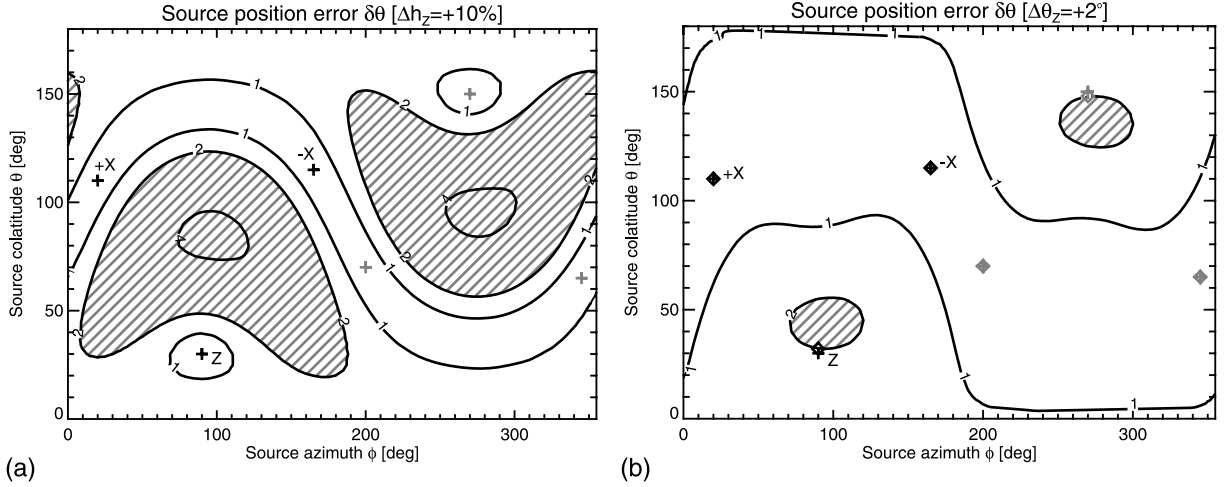
Figure 10. Error on the source position \delta\theta introduced by (a) a +10% bias on the Z antenna length h_Z , and (b) a +2^\circ bias on the Z antenna colatitude \theta_Z . Coordinates are in the spacecraft frame. The region in which \delta\theta > 2^\circ has been hatched. The crosses and the diamonds represent, respectively, the input and biased the antenna directions. Boldface symbols correspond to the antenna direction, lightface ones to the opposite directions. Lines are isocontours in degree.
