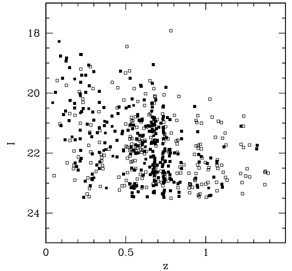
Fig. 7. The variation in the apparent I magnitude as a function of redshift for galaxies for which redshifts are measured by the IMAGES survey. Filled and open squares show secure and insecure redshift estimates, respectively.
