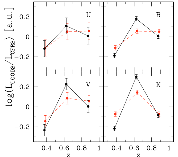
Fig. 12. Evolution in the ratios of luminosity densities of observed galaxies from the GOODS spectroscopic sample and observed galaxies from CFRS as a function of redshift, for 3 redshift bins (0.25–0.5; 0.5–0.75, and 0.75–1). Black and red-dashed lines correspond to values calculated using the spectroscopic and photometric redshifts, respectively.
