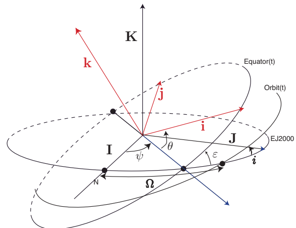
Fig. 1. The orbital plane is defined by the inclination i and longitude of node \Omega with respect to a fixed reference frame (I, J, K) , while (i, j, k) are the axis of inertia of the planet.
