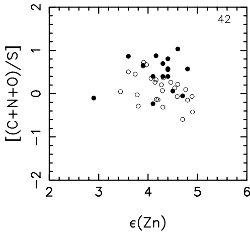
Fig. 8. [(C+N+O)/S] as a function of the metallicity as measured by \epsilon(Zn) .
