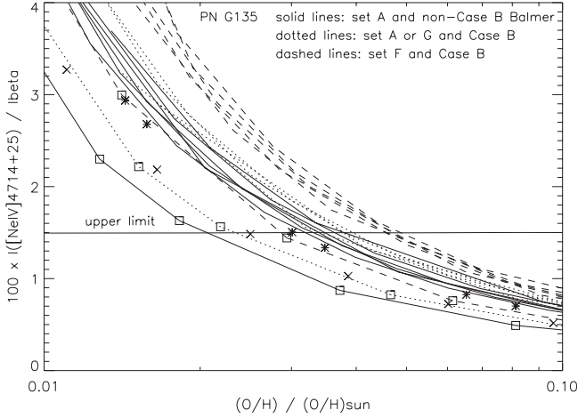
Fig. 14. Predicted intensity of multiplet [\text{Ne IV}]\lambda 4714+25 versus \text{O}/\text{H} in solar units for all model sequences. Dashed and dotted lines: Case B model sequences using data sets F and G or A respectively. Solid lines: non-Case B model sequences using data set A. Asterisks: variants of non-Case B D10C1A and D10C7A models with covering factor f = 0.5 . Squares, linked by dashed, dotted, or solid lines (as above): variants with pre-Nahar oxygen recombination coefficients. Multiplication crosses: variants of D10C1A with modified \text{Ne}^{3+} recombination.
