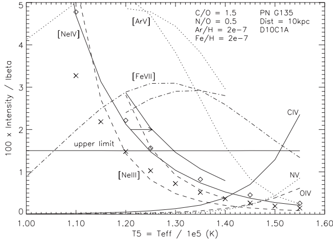
Fig. 10. Predicted intensities in units I_{H\beta} = 100 versus T_{\text{eff}} for optical lines in model sequence D10C1A and some variants. The forbidden lines are [Ne III] 3869+3968, [Ne IV] 4714+25, [Ar V] 7005+6435 and [Fe VII] 6087 and the permitted lines are CIV 4658, O IV 4632 and N V 4945. Curves for [Ar V] and [Fe VII] correspond to fixed abundances. Horizontal line I = 1.5 : upper limit 1–1.5 adopted for these lines. Shifted curves drawn from T_5 = 1.2 –1.4: variant of D10C1A in which f = 0.5 ; an horizontal arrow indicates the shift for [Ne IV]. Diamonds and crosses: [Ne IV] intensity for variants in which either \text{O}^{2+} – \text{O}^{4+} or \text{Ne}^{3+} have modified recombination coefficients (Sect. 4.3.1).
