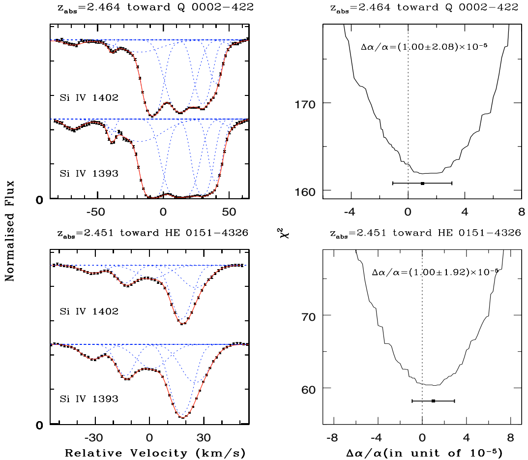
Fig. 5. Left panels show on a velocity scale Si IV doublet data points with error-bars together with the best Voigt-profile fit for \Delta\alpha/\alpha = 0 over plotted as a solid line. The Voigt profiles of individual sub-components are shown by dashed lines. Right panels show the variation of \chi^2 as a function of \Delta\alpha/\alpha . The dark rectangle with error bars indicates the measured value of \Delta\alpha/\alpha with one sigma error-bars derived using the criteria \Delta\chi^2 = 1 around the minima. The name of QSOs, z_{\text{abs}} and the value of measured \Delta\alpha/\alpha are also stated explicitly.
