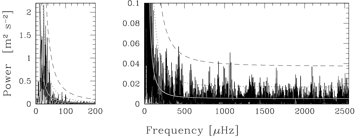
Fig. 2. Power spectrum of HD 209625 ( right ), with a zoom on the low-frequency part ( left ). The white line indicates the mean noise level, while dotted and dashed lines represent an amplitude of 2\sigma and 3\sigma respectively.
