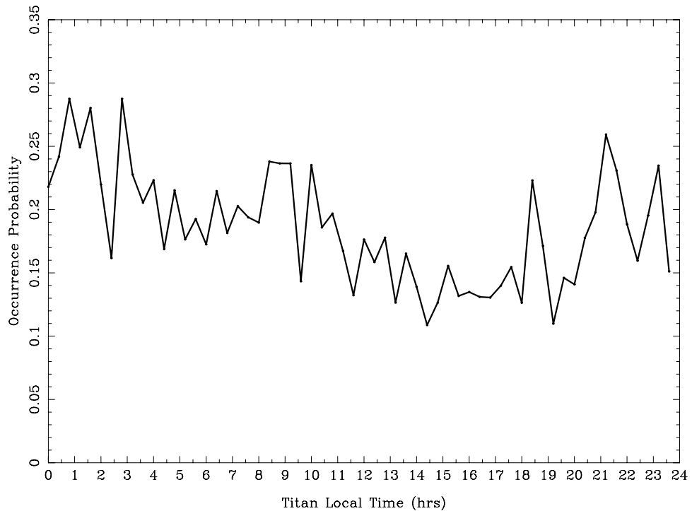
Figure 5. Plot of OP averaged over the range 20^\circ < SSSL < 180^\circ versus Titan LT.
