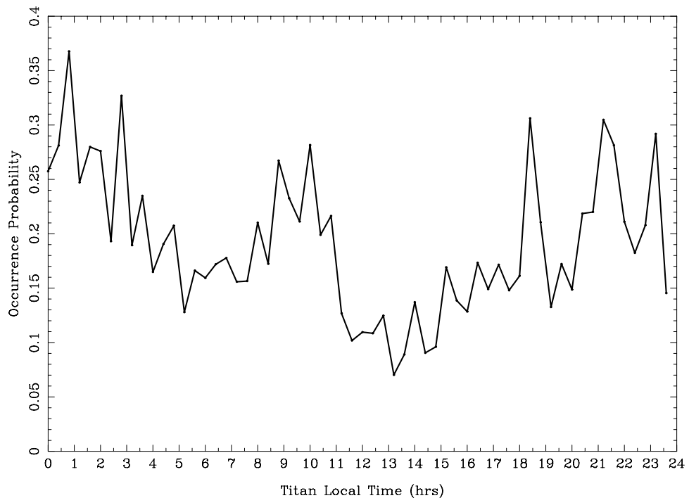
Figure 8. Plot of OP averaged over the range 0^\circ < SSSL < 200^\circ versus Titan LT.
