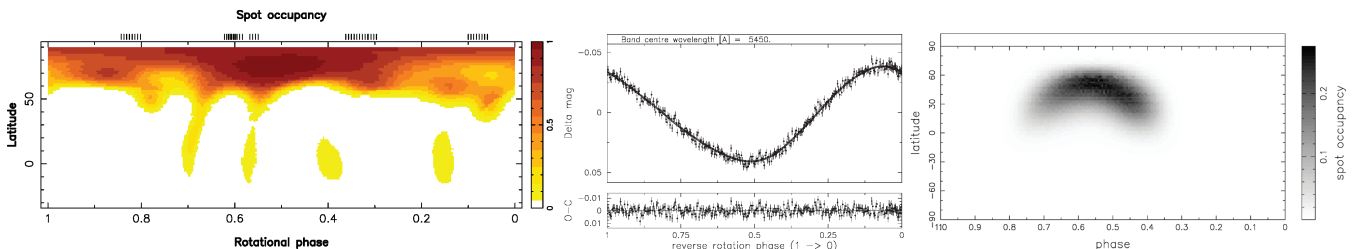
Figure 11. The original spot distribution (left) of HD 171488 reconstructed using Doppler imaging for 2007 November (Fig 1: middle panel). This was used as input to the light-curve modelling program DORS , from which the light curve shown in the middle panel was computed. This light curve was then used as the only input to the light-curve inversion code. The reconstructed surface brightness image from the light curve is shown to the right.
