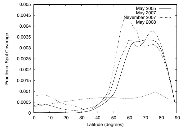
Figure 4. Fractional spot coverage per latitude bin integrated over longitude for all epochs of this analysis. For comparison, the fractional spottedness is also shown for 2005 May.
