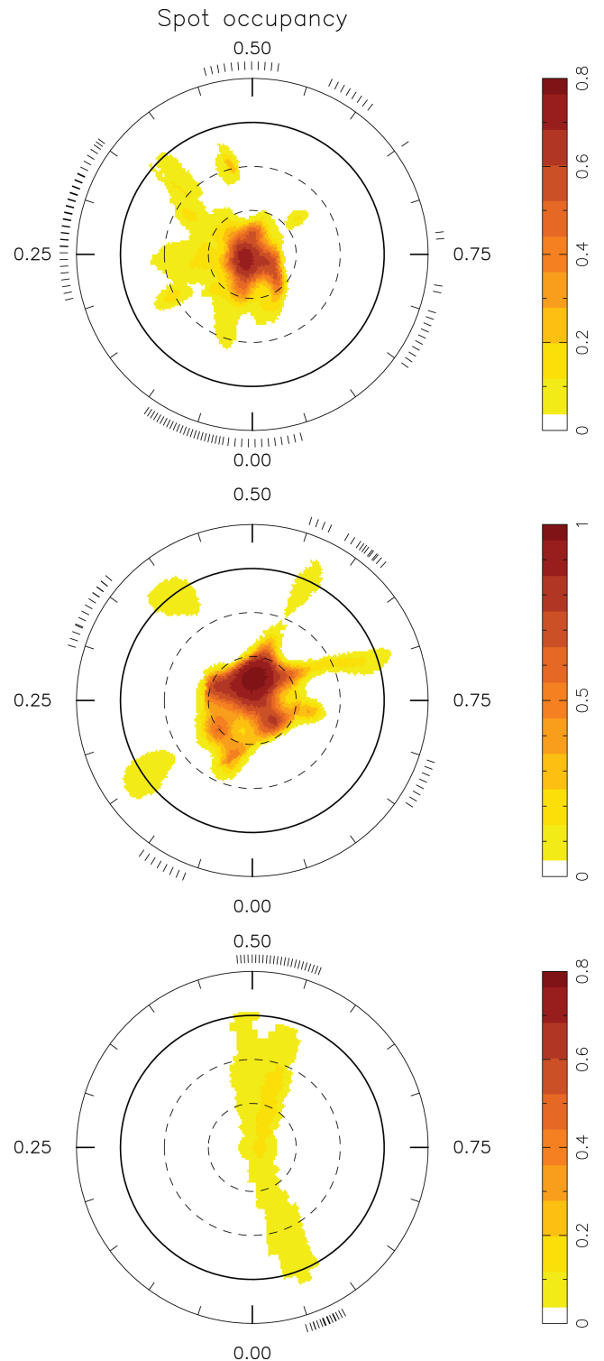
Figure 1. Maximum entropy brightness maps for HD 171488 in 2007 May (top), 2007 November (middle) and 2008 May (bottom). These images are flattened polar projections extending down to a latitude of -30^\circ , where the bold line depicts the equator and the dashed lines are at 30^\circ intervals. The radial ticks surrounding each image indicate the rotational phase of individual Stokes I observations. The images shown here include the values for differential rotation measured in Section 4 to avoid smearing of spots over the long phase coverage of our data sets.
