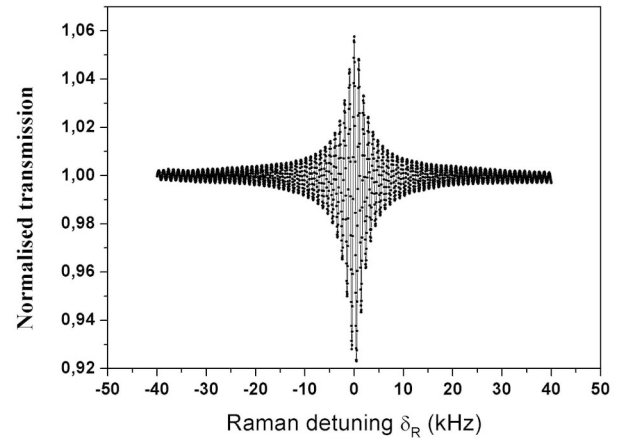
FIG. 6. Experimental saturated Raman-Ramsey fringes with total intensity \sim 500 \mu\text{W}/\text{cm}^2 . The first pulse duration is \tau_1 = 5 \text{ms} and the second pulse duration is \tau_2 = 5 \mu\text{s} ; 8 average scan.
