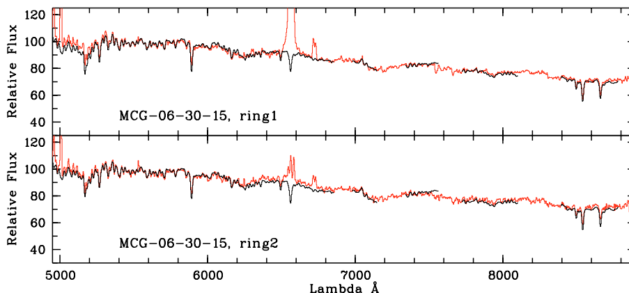
Fig. 8. MCG-06-30-15: synthetic spectrum (black line) superimposed on the dereddened observed spectrum (grey line). Top: spectrum of a ring at 360 pc from the nucleus. Bottom: spectrum of a ring at 650 pc from the nucleus.
