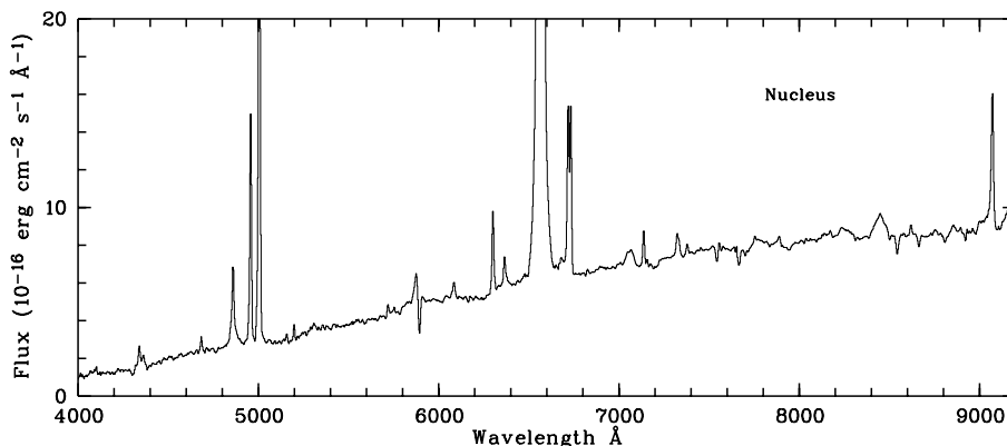
Fig. 1. Nuclear spectrum of the Seyfert 1.9 NGC 2992. Note the prominent broad OI 8446 Å emission.
