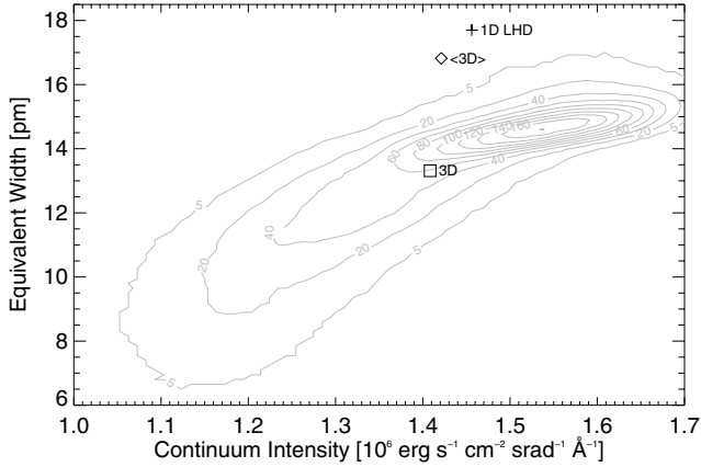
Fig. 3. Procyon: joint probability density function (not normalised) of continuum intensity and (disk-centre) EW for the 1045.9 nm line in the 3D model (grey contours). The labelled symbols mark the 3D and \langle 3D \rangle average, as well as the result for a LHD model with \alpha_{\text{MLT}} = 1.5 . The micro-turbulent velocity for the 1D models is 2.1 \text{ km s}^{-1} .
