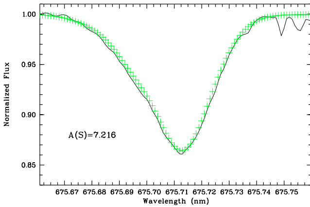
Fig. 2. Procyon: the 3D fit (green/grey crosses) is super imposed on the observed spectrum (black solid line) for the S I 675.7 nm triplet.
