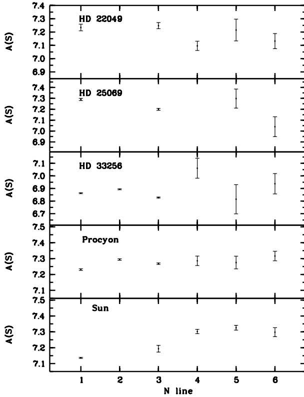
Fig. 6. For each star, A (S) plotted as a function of the number of the line: 1 is the 675.7 nm triplet, 2 the 869.3 nm line, 3 the 869.4 nm line, 4 the 1045.5 nm line, 5 the 1045.6 nm line, and 6 the 1045.9 nm line. For the Sun, the error bar is related to the statistical error coming from the two observed flux spectra. For the other stars, it is related to the S/N through Eq. (1).
