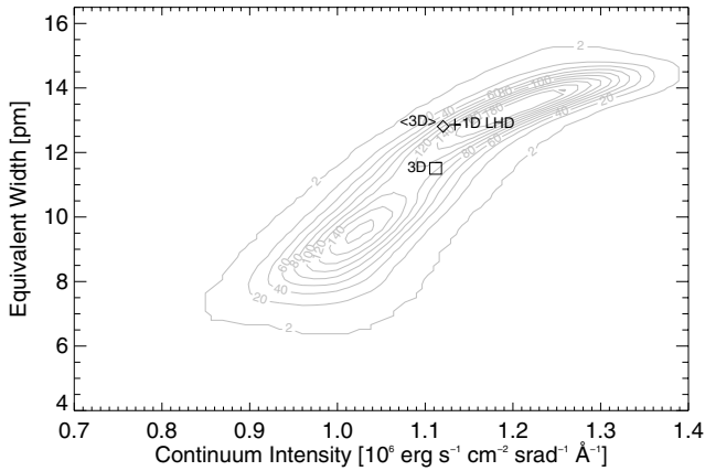
Fig. 4. Sun: same as Fig. 3 for the solar case. The micro-turbulent velocity for the 1D models is 1.0 \text{ km s}^{-1} .
