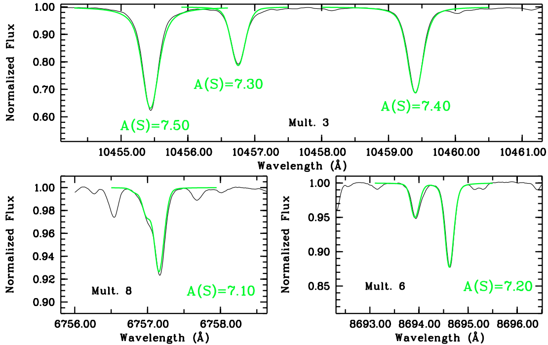
Fig. 1. Sun: synthetic spectra (green/grey thick solid line) based on the 3D model atmosphere are super imposed on the observed (black solid line) solar flux spectrum of Kurucz.
