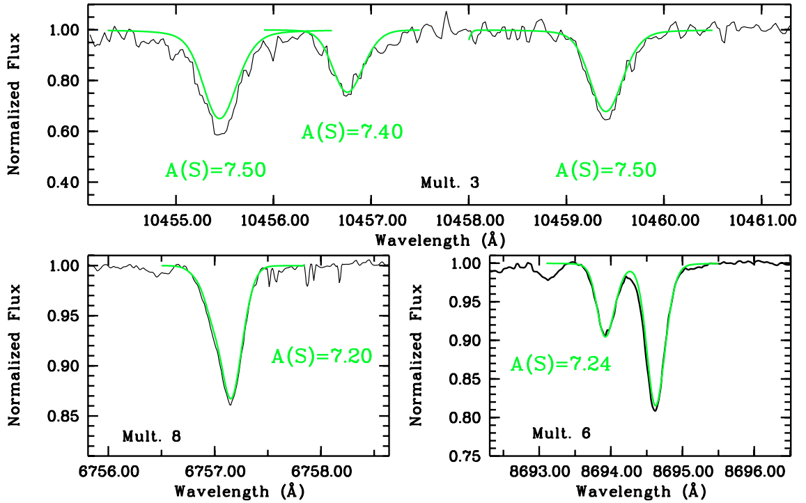
Fig. 5. Procyon: synthetic spectra (green thick line) based on the 3D model are super imposed on the observed (black solid line) ones.
